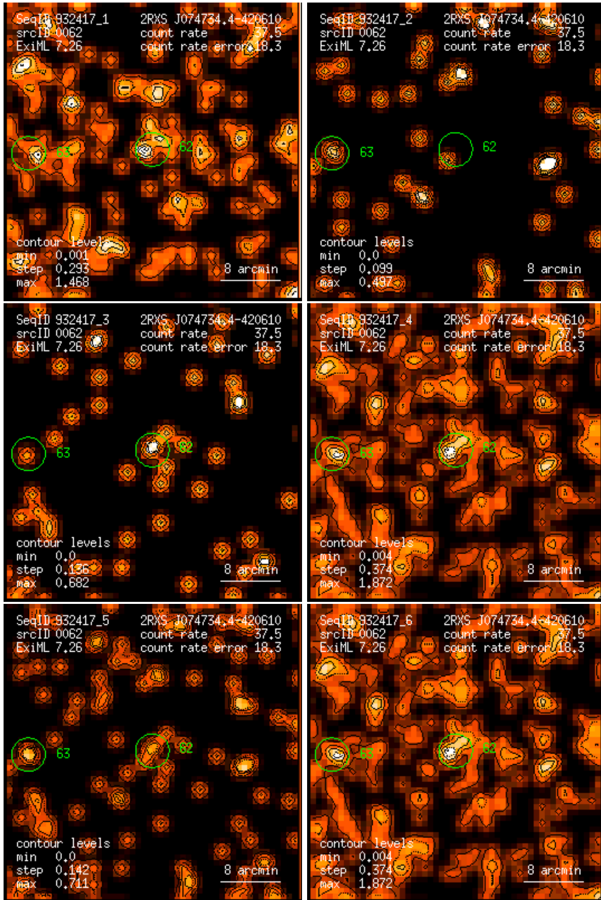
Figure 62: RASS 932417: detection 0062: band rate images, Gaussian filter: (1) PSPC channels 11 – 41, (2) 52 – 90, (3) 91 – 201, (4) 11 – 235, (5) 52 – 201, (6) 11 – 201. Broad band rates in counts/ks. Band rate contour levels in counts/ks/arcmin 2 .
