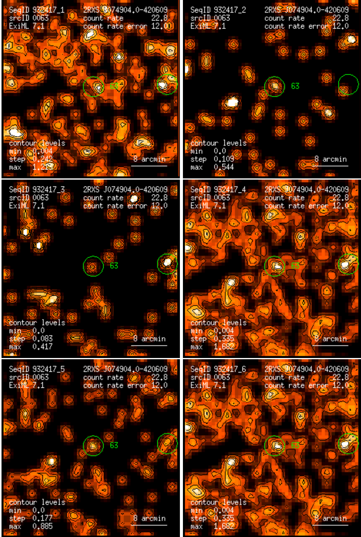
Figure 63: RASS 932417: detection 0063: band rate images, Gaussian filter: (1) PSPC channels 11 – 41, (2) 52 – 90, (3) 91 – 201, (4) 11 – 235, (5) 52 – 201, (6) 11 – 201. Broad band rates in counts/ks. Band rate contour levels in counts/ks/arcmin 2 .
