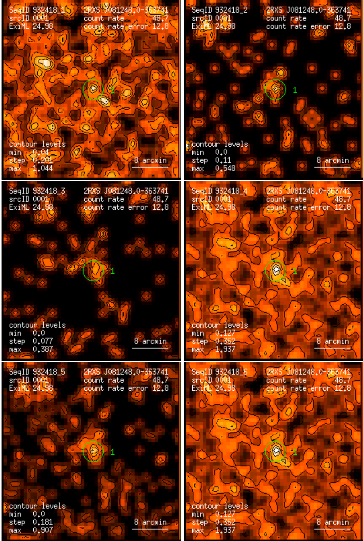
Figure 1: RASS 932418: detection 0001: band rate images, Gaussian filter: (1) PSPC channels 11 – 41, (2) 52 – 90, (3) 91 – 201, (4) 11 – 235, (5) 52 – 201, (6) 11 – 201. Broad band rates in counts/ks. Band rate contour levels in counts/ks/arcmin 2 .
