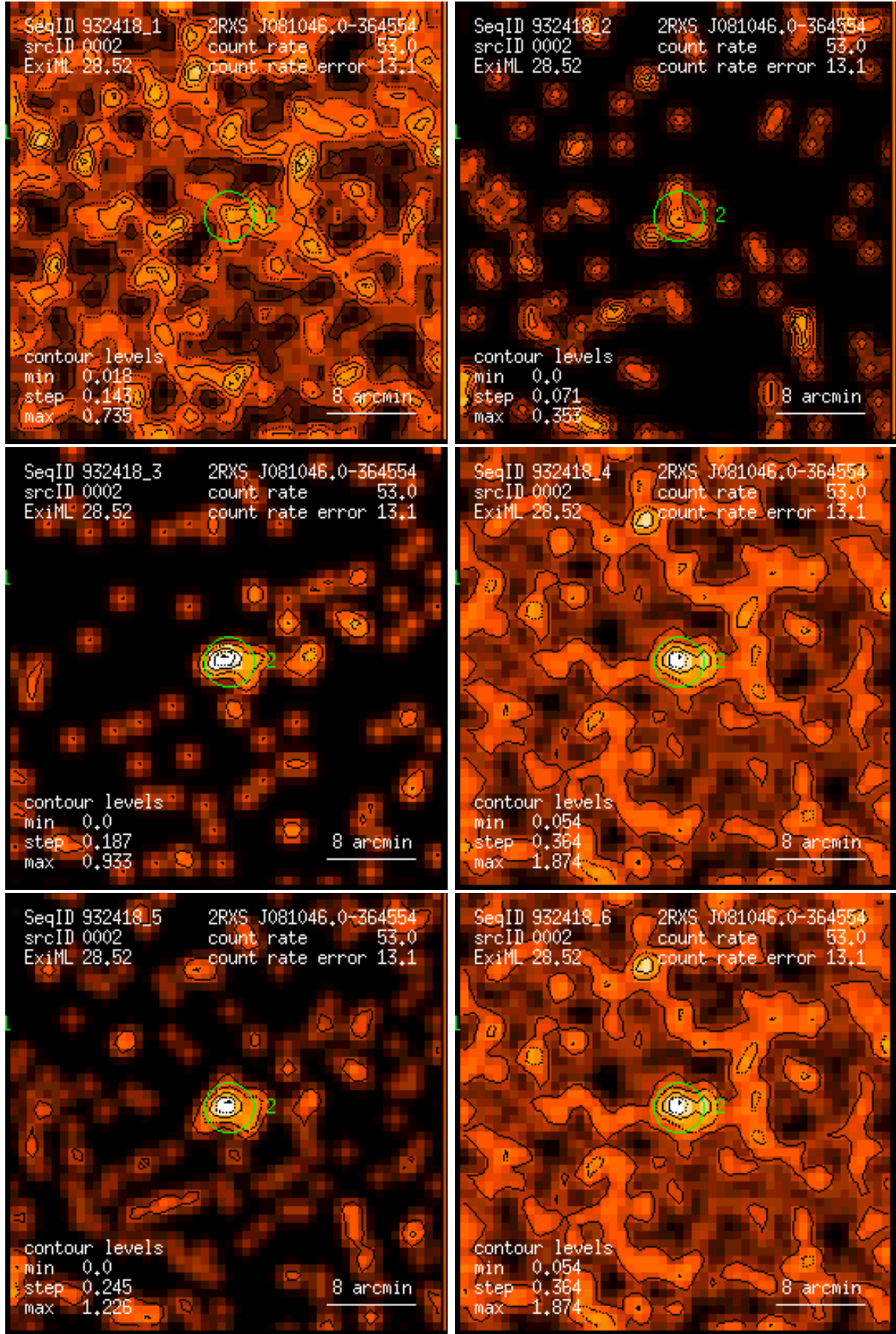
Figure 2: RASS 932418: detection 0002: band rate images, Gaussian filter: (1) PSPC channels 11 – 41, (2) 52 – 90, (3) 91 – 201, (4) 11 – 235, (5) 52 – 201, (6) 11 – 201. Broad band rates in counts/ks. Band rate contour levels in counts/ks/arcmin 2 .
