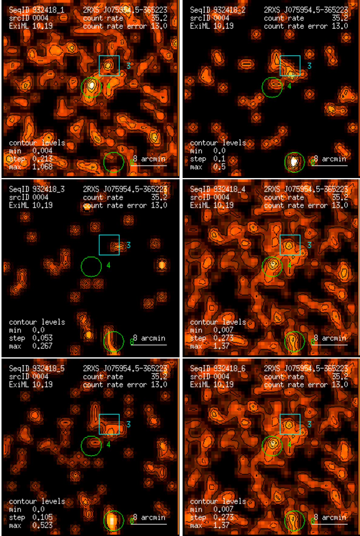
Figure 4: RASS 932418: detection 0004: band rate images, Gaussian filter: (1) PSPC channels 11 – 41, (2) 52 – 90, (3) 91 – 201, (4) 11 – 235, (5) 52 – 201, (6) 11 – 201. Broad band rates in counts/ks. Band rate contour levels in counts/ks/arcmin 2 .
