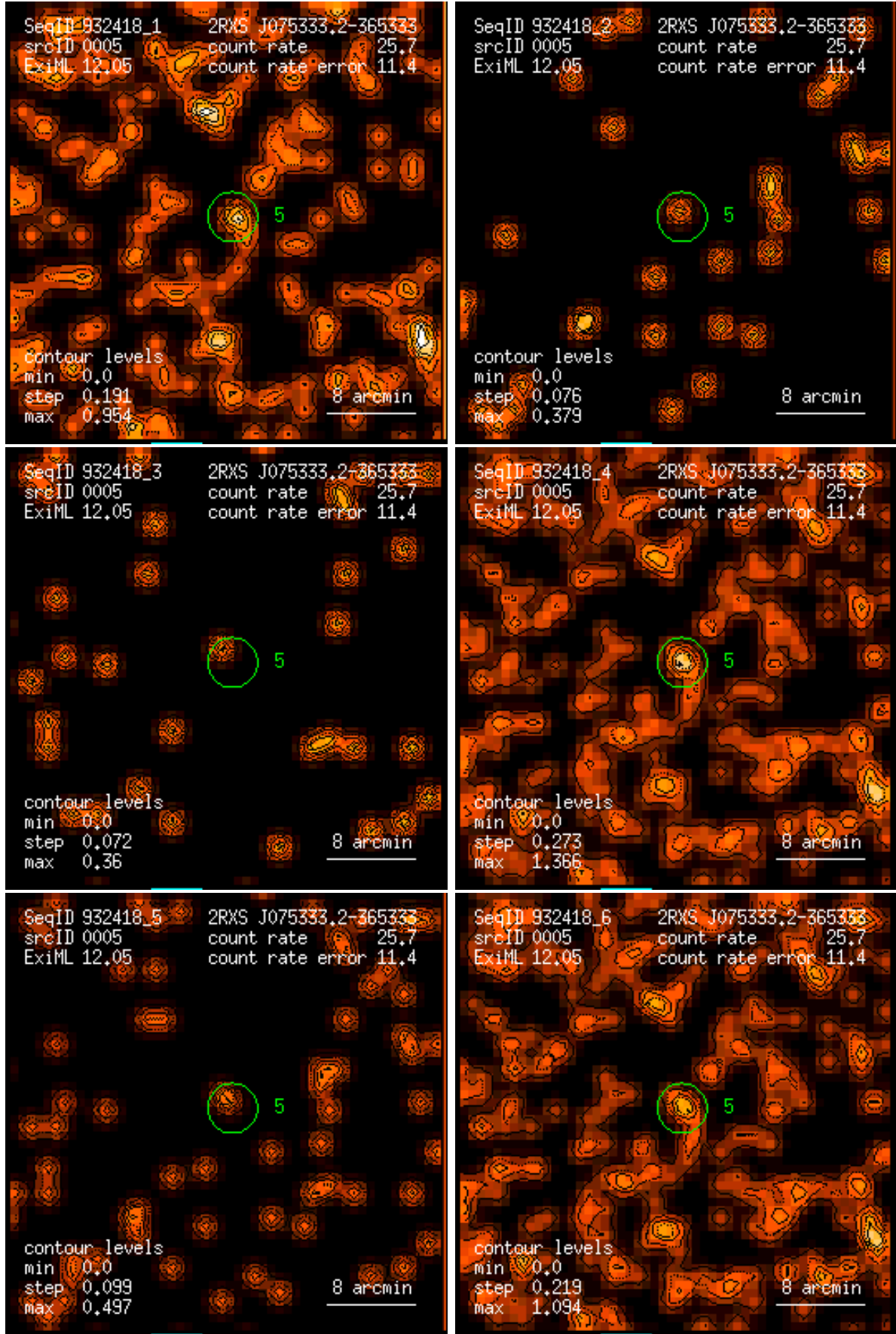
Figure 5: RASS 932418: detection 0005: band rate images, Gaussian filter: (1) PSPC channels 11 – 41, (2) 52 – 90, (3) 91 – 201, (4) 11 – 235, (5) 52 – 201, (6) 11 – 201. Broad band rates in counts/ks. Band rate contour levels in counts/ks/arcmin 2 .
