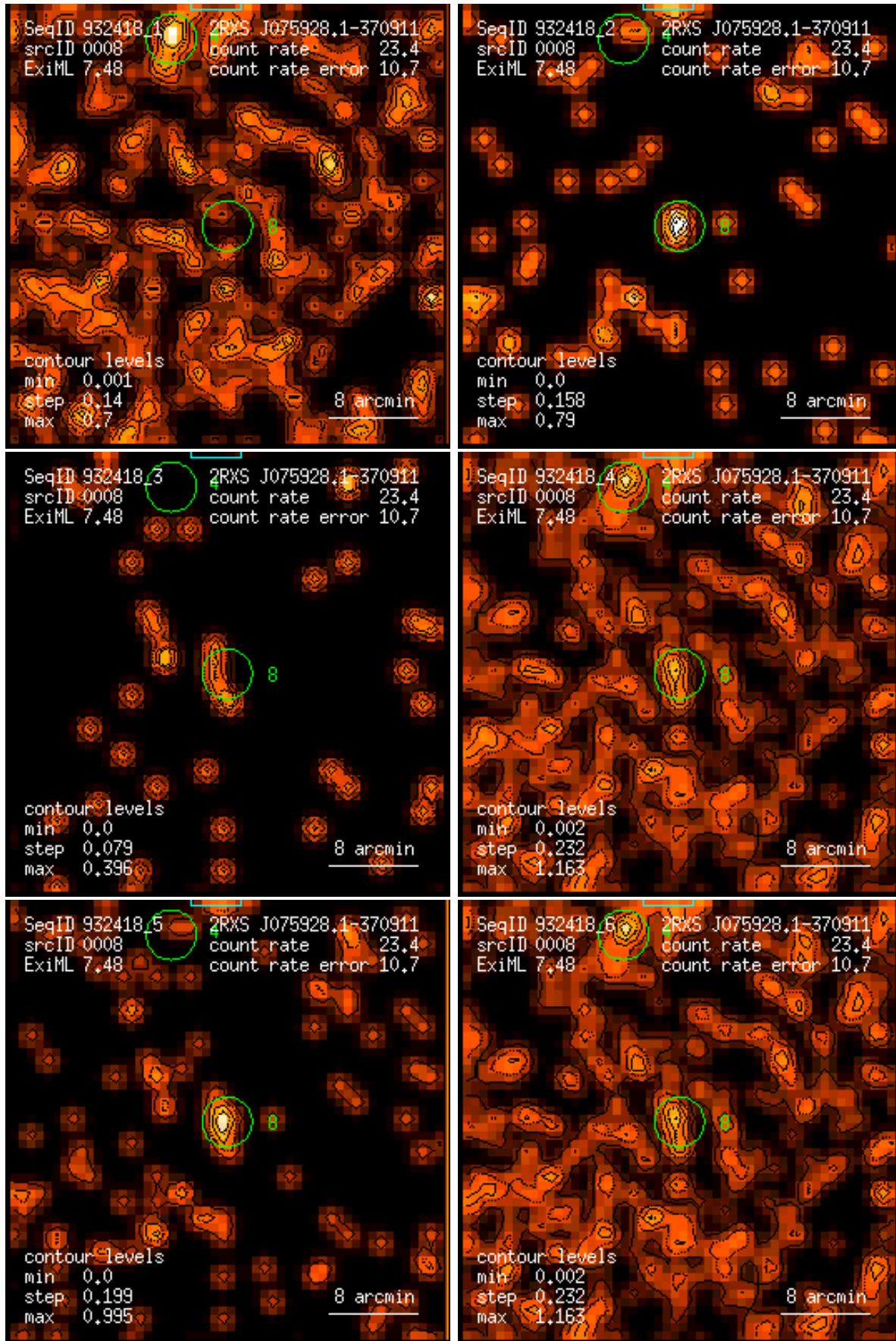
Figure 8: RASS 932418: detection 0008: band rate images, Gaussian filter: (1) PSPC channels 11 – 41, (2) 52 – 90, (3) 91 – 201, (4) 11 – 235, (5) 52 – 201, (6) 11 – 201. Broad band rates in counts/ks. Band rate contour levels in counts/ks/arcmin 2 .
