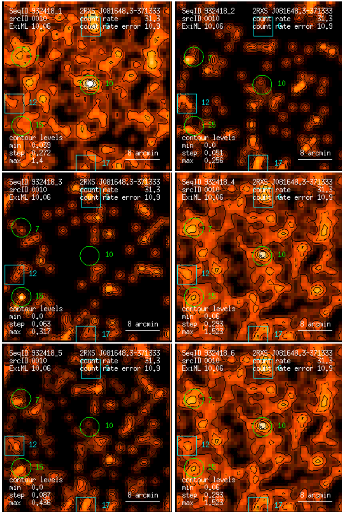
Figure 10: RASS 932418: detection 0010: band rate images, Gaussian filter: (1) PSPC channels 11 – 41, (2) 52 – 90, (3) 91 – 201, (4) 11 – 235, (5) 52 – 201, (6) 11 – 201. Broad band rates in counts/ks. Band rate contour levels in counts/ks/arcmin 2 .
