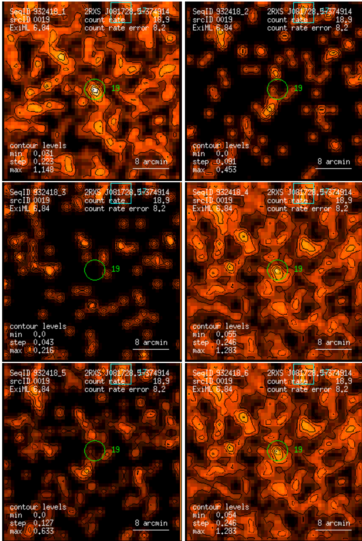
Figure 19: RASS 932418: detection 0019: band rate images, Gaussian filter: (1) PSPC channels 11 – 41, (2) 52 – 90, (3) 91 – 201, (4) 11 – 235, (5) 52 – 201, (6) 11 – 201. Broad band rates in counts/ks. Band rate contour levels in counts/ks/arcmin 2 .
