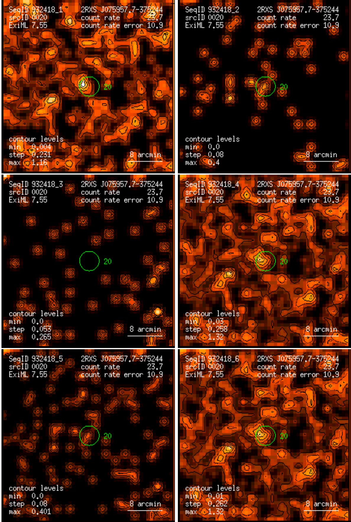
Figure 20: RASS 932418: detection 0020: band rate images, Gaussian filter: (1) PSPC channels 11 – 41, (2) 52 – 90, (3) 91 – 201, (4) 11 – 235, (5) 52 – 201, (6) 11 – 201. Broad band rates in counts/ks. Band rate contour levels in counts/ks/arcmin 2 .
