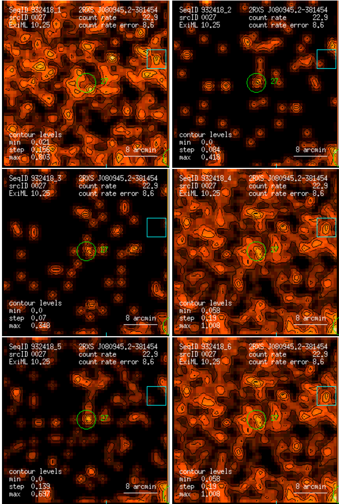
Figure 27: RASS 932418: detection 0027: band rate images, Gaussian filter: (1) PSPC channels 11 – 41, (2) 52 – 90, (3) 91 – 201, (4) 11 – 235, (5) 52 – 201, (6) 11 – 201. Broad band rates in counts/ks. Band rate contour levels in counts/ks/arcmin 2 .
