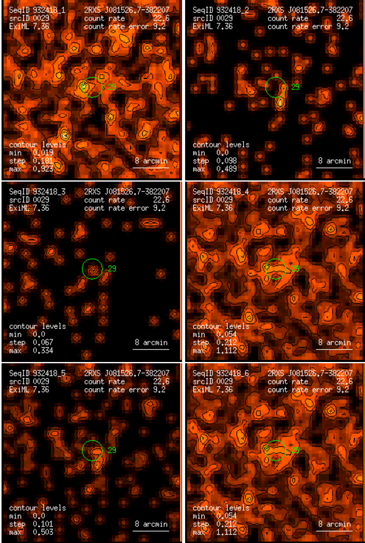
Figure 29: RASS 932418: detection 0029: band rate images, Gaussian filter: (1) PSPC channels 11 – 41, (2) 52 – 90, (3) 91 – 201, (4) 11 – 235, (5) 52 – 201, (6) 11 – 201. Broad band rates in counts/ks. Band rate contour levels in counts/ks/arcmin 2 .
