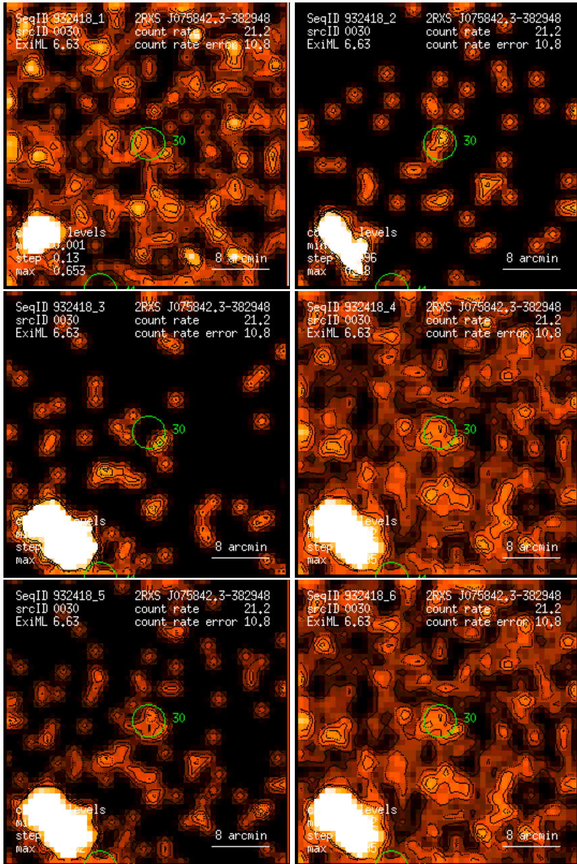
Figure 30: RASS 932418: detection 0030: band rate images, Gaussian filter: (1) PSPC channels 11 – 41, (2) 52 – 90, (3) 91 – 201, (4) 11 – 235, (5) 52 – 201, (6) 11 – 201. Broad band rates in counts/ks. Band rate contour levels in counts/ks/arcmin 2 .
