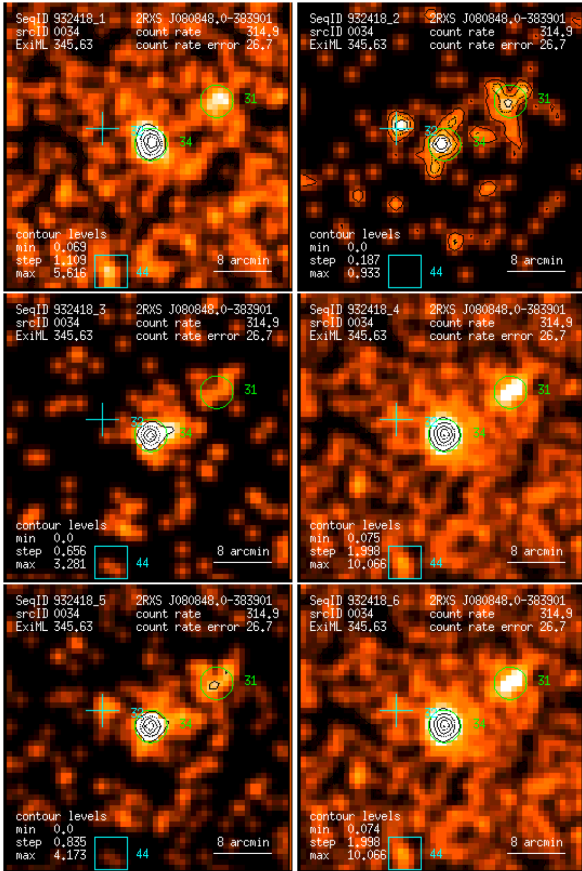
Figure 34: RASS 932418: detection 0034: band rate images, Gaussian filter: (1) PSPC channels 11 – 41, (2) 52 – 90, (3) 91 – 201, (4) 11 – 235, (5) 52 – 201, (6) 11 – 201. Broad band rates in counts/ks. Band rate contour levels in counts/ks/arcmin 2 .
