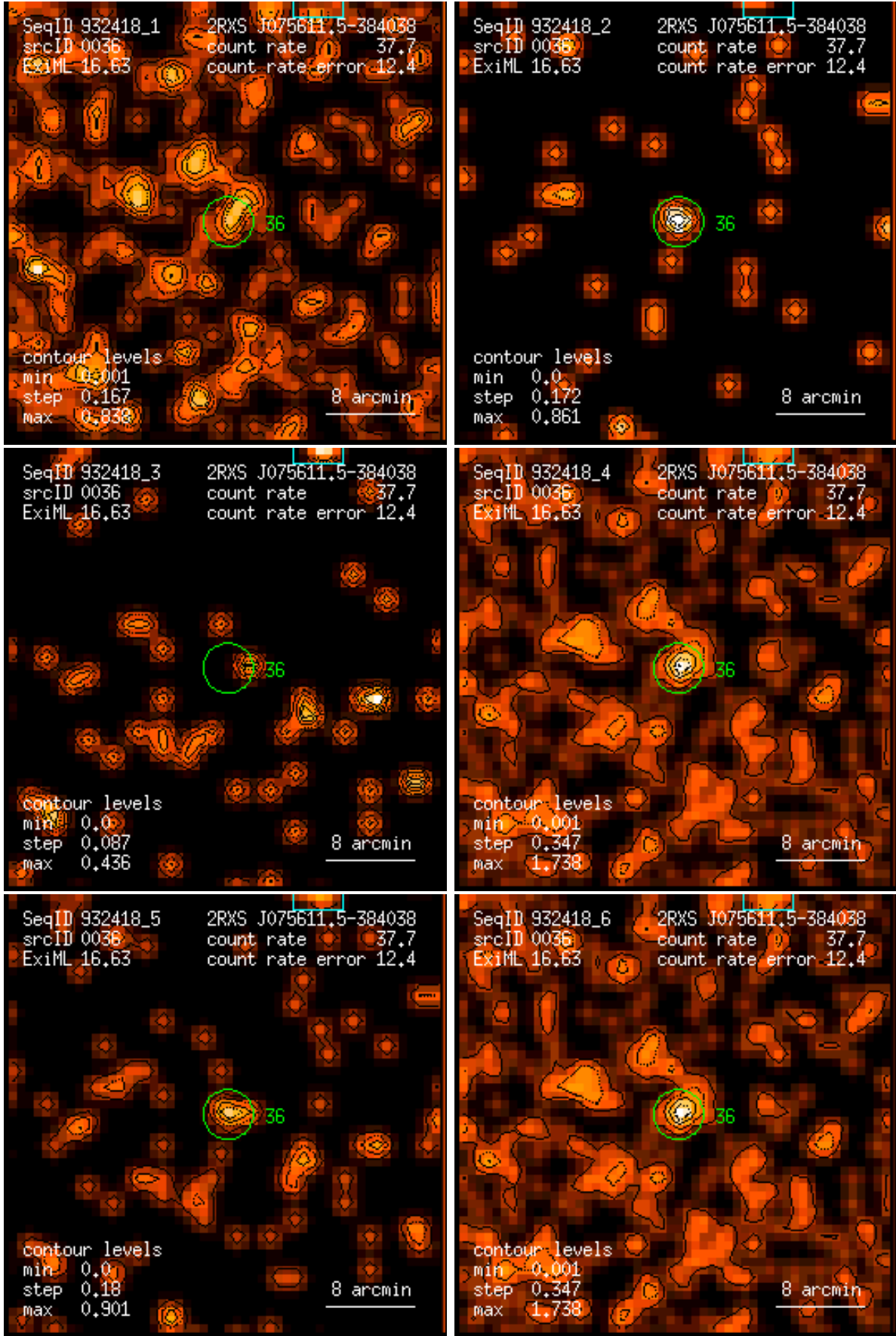
Figure 36: RASS 932418: detection 0036: band rate images, Gaussian filter: (1) PSPC channels 11 – 41, (2) 52 – 90, (3) 91 – 201, (4) 11 – 235, (5) 52 – 201, (6) 11 – 201. Broad band rates in counts/ks. Band rate contour levels in counts/ks/arcmin 2 .
