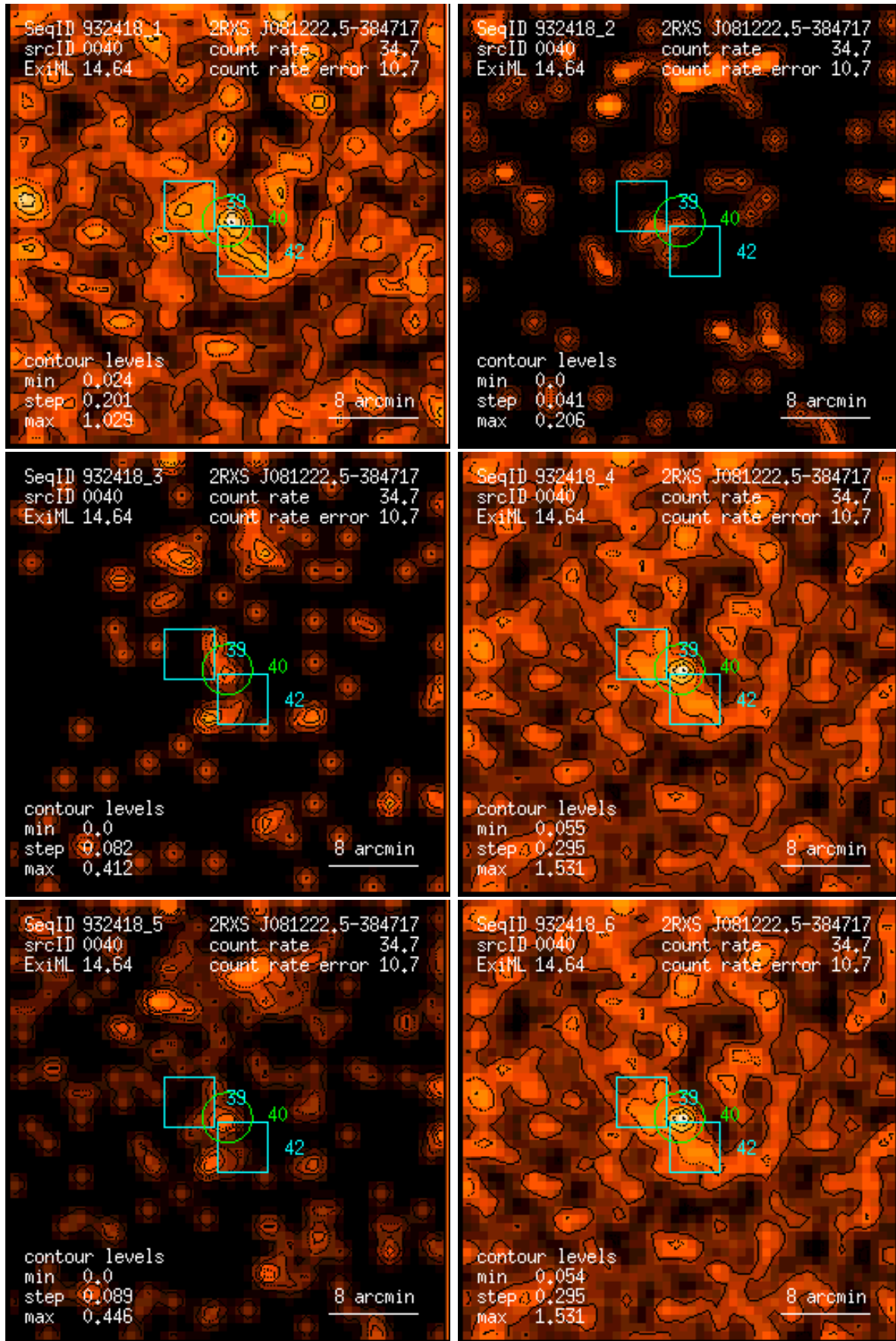
Figure 40: RASS 932418: detection 0040: band rate images, Gaussian filter: (1) PSPC channels 11 – 41, (2) 52 – 90, (3) 91 – 201, (4) 11 – 235, (5) 52 – 201, (6) 11 – 201. Broad band rates in counts/ks. Band rate contour levels in counts/ks/arcmin 2 .
