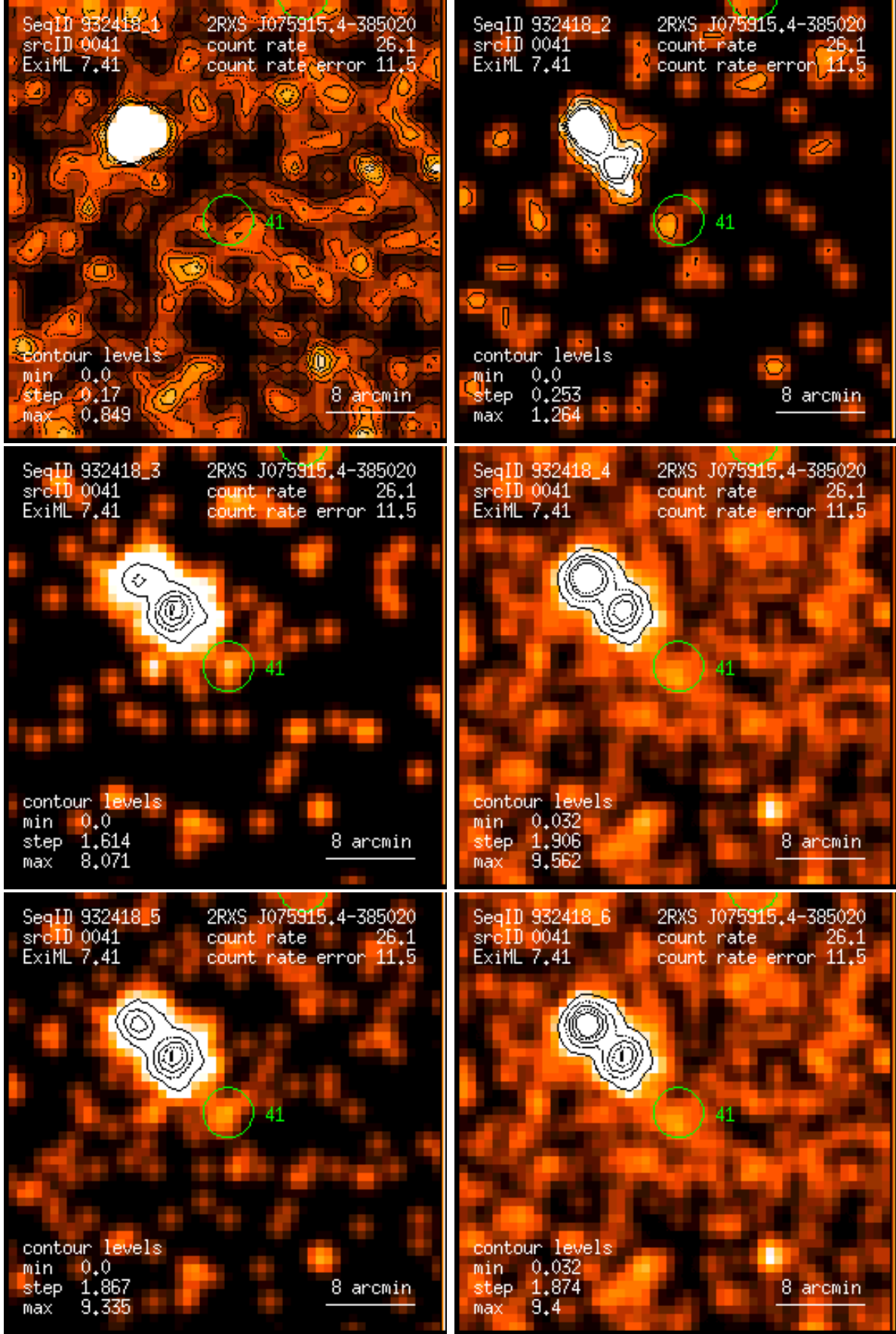
Figure 41: RASS 932418: detection 0041: band rate images, Gaussian filter: (1) PSPC channels 11 – 41, (2) 52 – 90, (3) 91 – 201, (4) 11 – 235, (5) 52 – 201, (6) 11 – 201. Broad band rates in counts/ks. Band rate contour levels in counts/ks/arcmin 2 .
