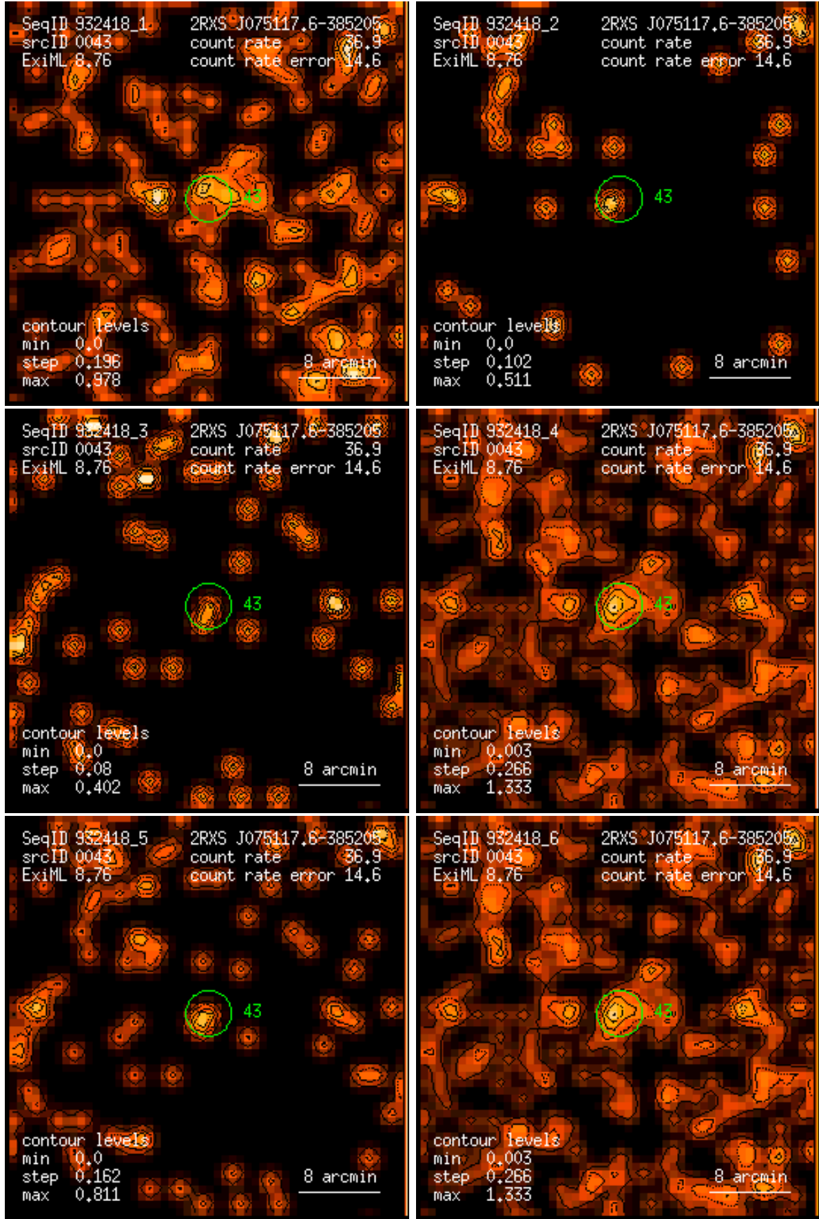
Figure 43: RASS 932418: detection 0043: band rate images, Gaussian filter: (1) PSPC channels 11 – 41, (2) 52 – 90, (3) 91 – 201, (4) 11 – 235, (5) 52 – 201, (6) 11 – 201. Broad band rates in counts/ks. Band rate contour levels in counts/ks/arcmin 2 .
