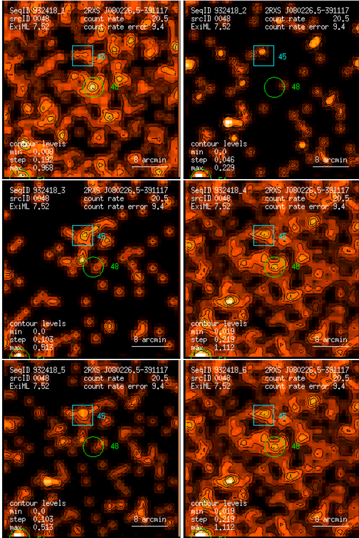
Figure 48: RASS 932418: detection 0048: band rate images, Gaussian filter: (1) PSPC channels 11 – 41, (2) 52 – 90, (3) 91 – 201, (4) 11 – 235, (5) 52 – 201, (6) 11 – 201. Broad band rates in counts/ks. Band rate contour levels in counts/ks/arcmin 2 .
