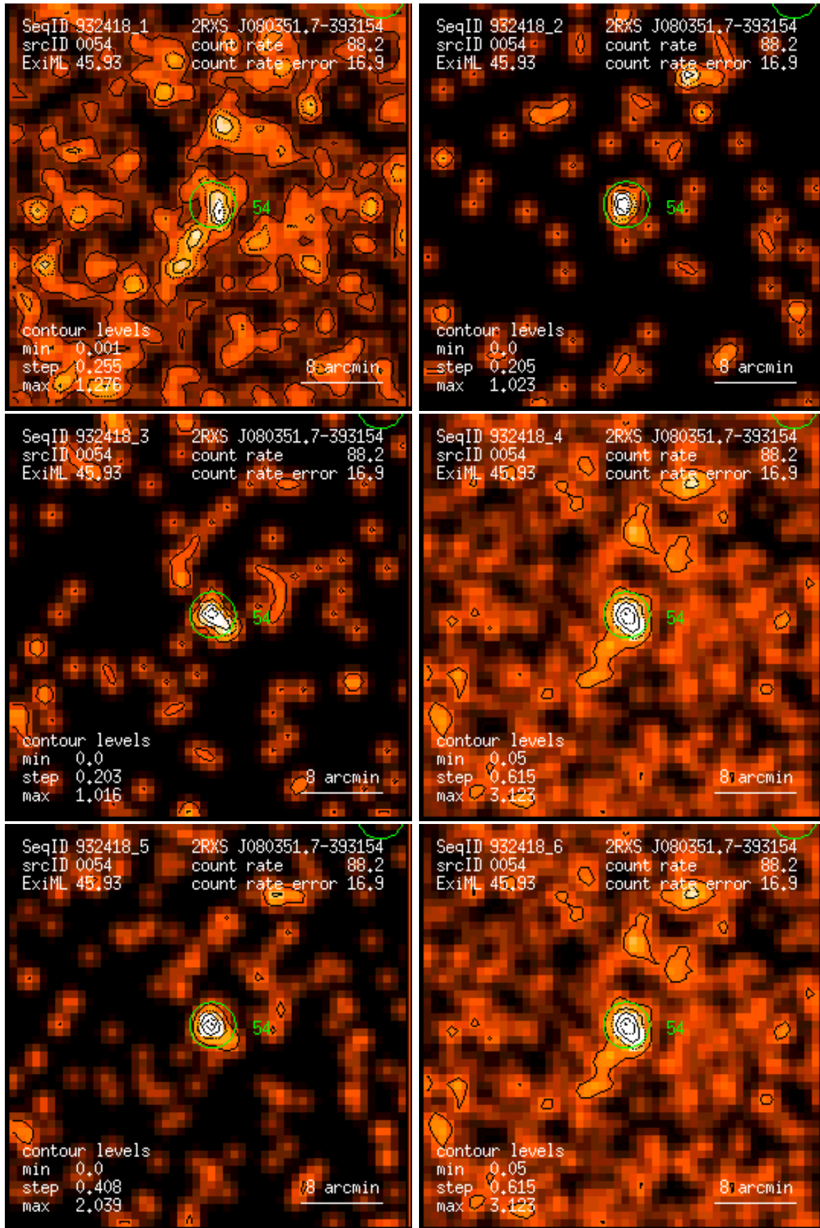
Figure 54: RASS 932418: detection 0054: band rate images, Gaussian filter: (1) PSPC channels 11 – 41, (2) 52 – 90, (3) 91 – 201, (4) 11 – 235, (5) 52 – 201, (6) 11 – 201. Broad band rates in counts/ks. Band rate contour levels in counts/ks/arcmin 2 .
