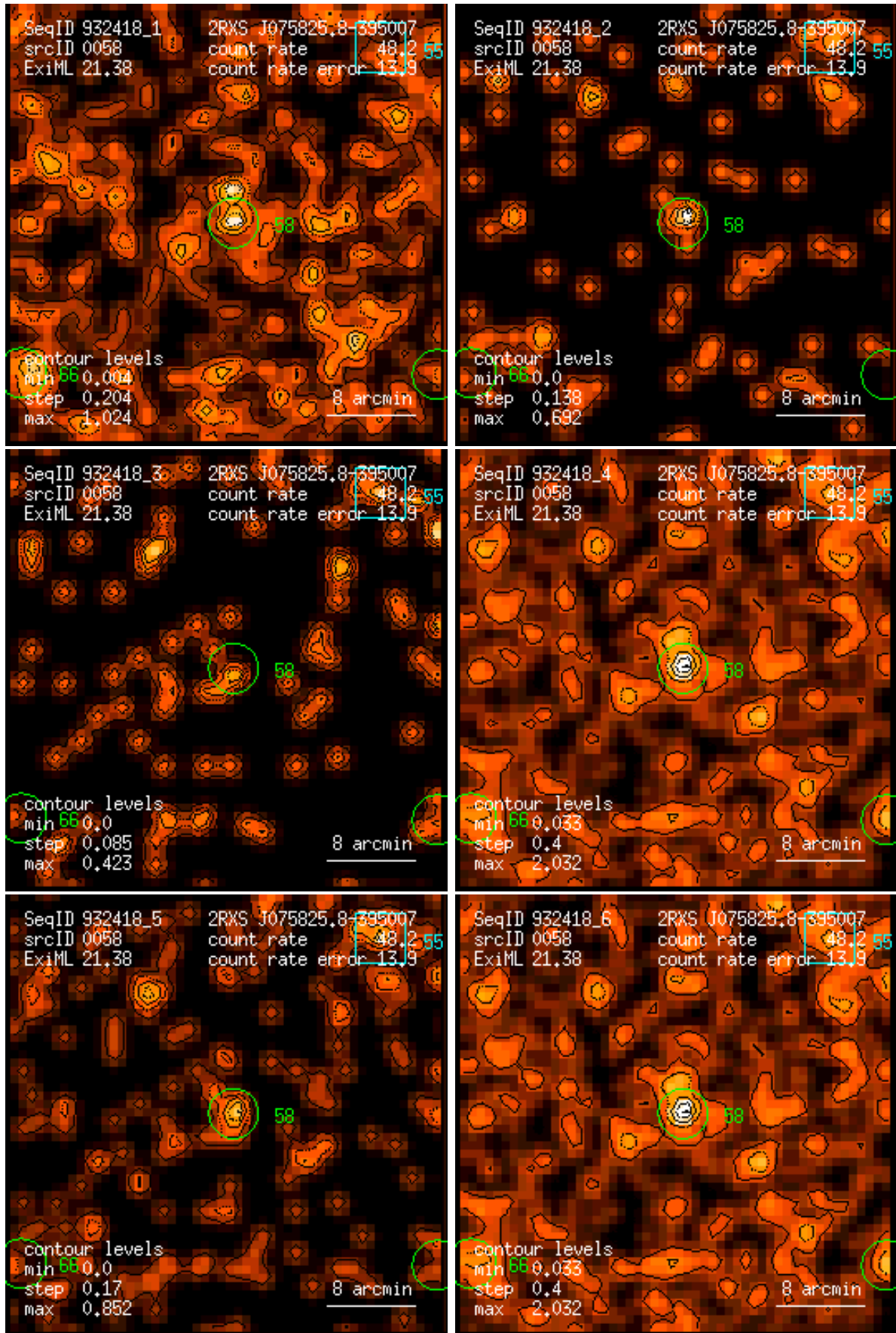
Figure 58: RASS 932418: detection 0058: band rate images, Gaussian filter: (1) PSPC channels 11 – 41, (2) 52 – 90, (3) 91 – 201, (4) 11 – 235, (5) 52 – 201, (6) 11 – 201. Broad band rates in counts/ks. Band rate contour levels in counts/ks/arcmin 2 .
