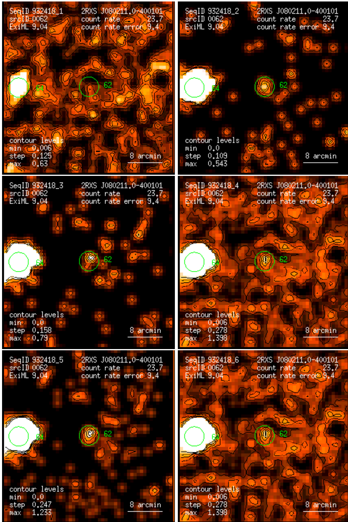
Figure 62: RASS 932418: detection 0062: band rate images, Gaussian filter: (1) PSPC channels 11 – 41, (2) 52 – 90, (3) 91 – 201, (4) 11 – 235, (5) 52 – 201, (6) 11 – 201. Broad band rates in counts/ks. Band rate contour levels in counts/ks/arcmin 2 .
