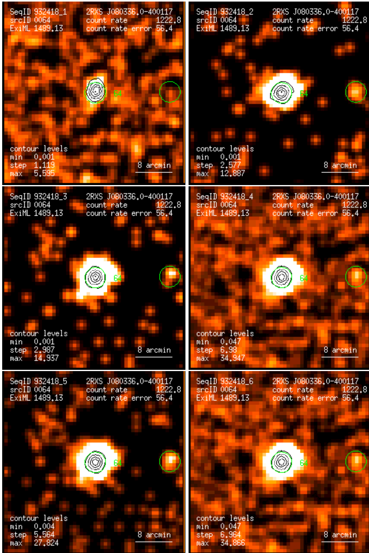
Figure 64: RASS 932418: detection 0064: band rate images, Gaussian filter: (1) PSPC channels 11 – 41, (2) 52 – 90, (3) 91 – 201, (4) 11 – 235, (5) 52 – 201, (6) 11 – 201. Broad band rates in counts/ks. Band rate contour levels in counts/ks/arcmin 2 .
