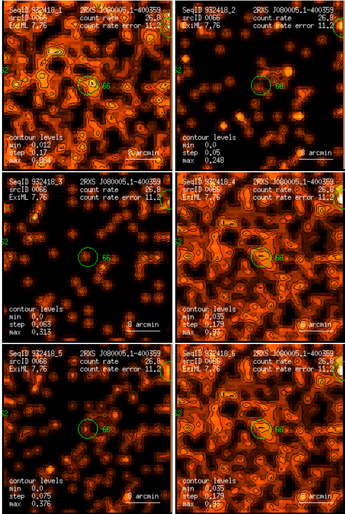
Figure 66: RASS 932418: detection 0066: band rate images, Gaussian filter: (1) PSPC channels 11 – 41, (2) 52 – 90, (3) 91 – 201, (4) 11 – 235, (5) 52 – 201, (6) 11 – 201. Broad band rates in counts/ks. Band rate contour levels in counts/ks/arcmin 2 .
