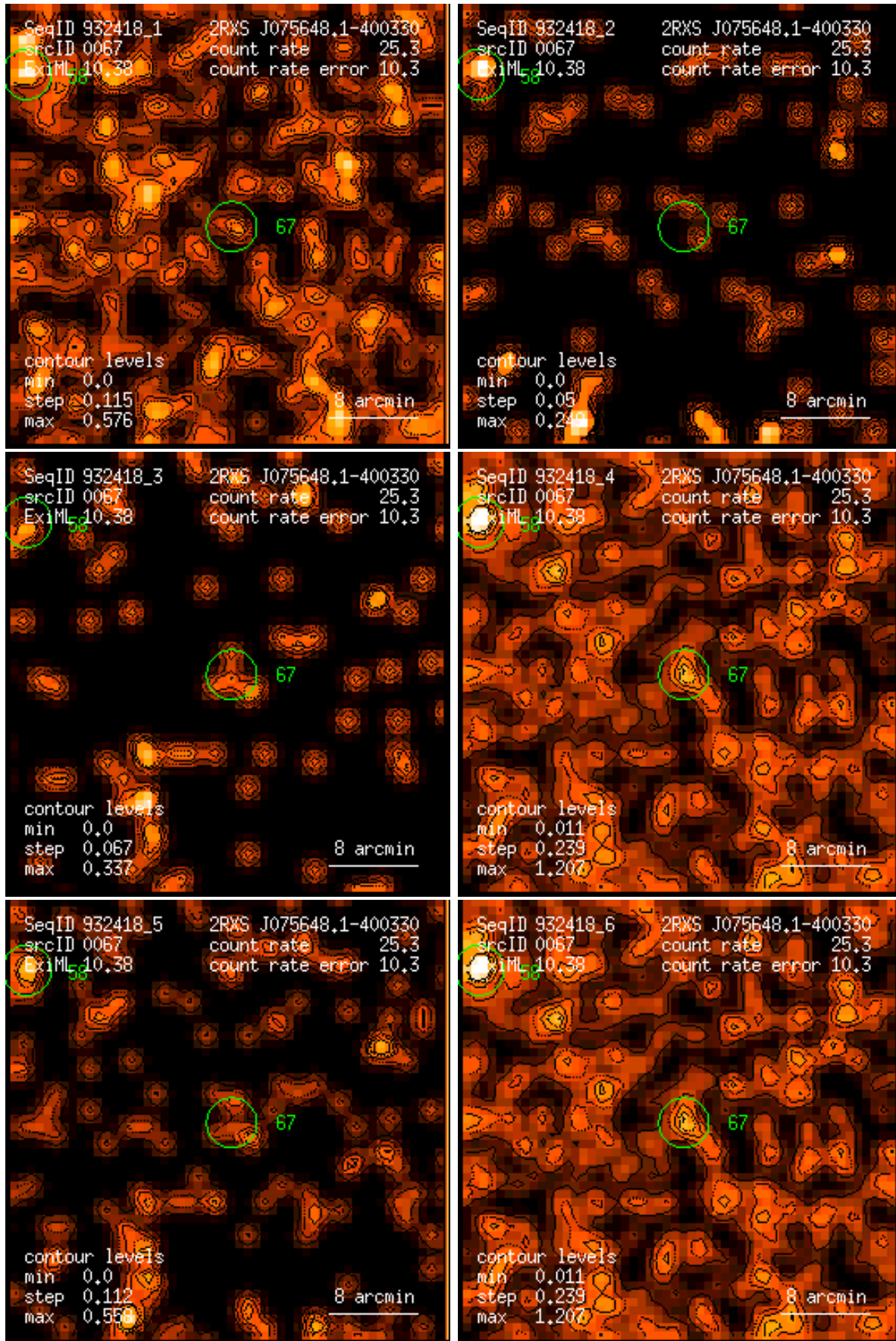
Figure 67: RASS 932418: detection 0067: band rate images, Gaussian filter: (1) PSPC channels 11 – 41, (2) 52 – 90, (3) 91 – 201, (4) 11 – 235, (5) 52 – 201, (6) 11 – 201. Broad band rates in counts/ks. Band rate contour levels in counts/ks/arcmin 2 .
