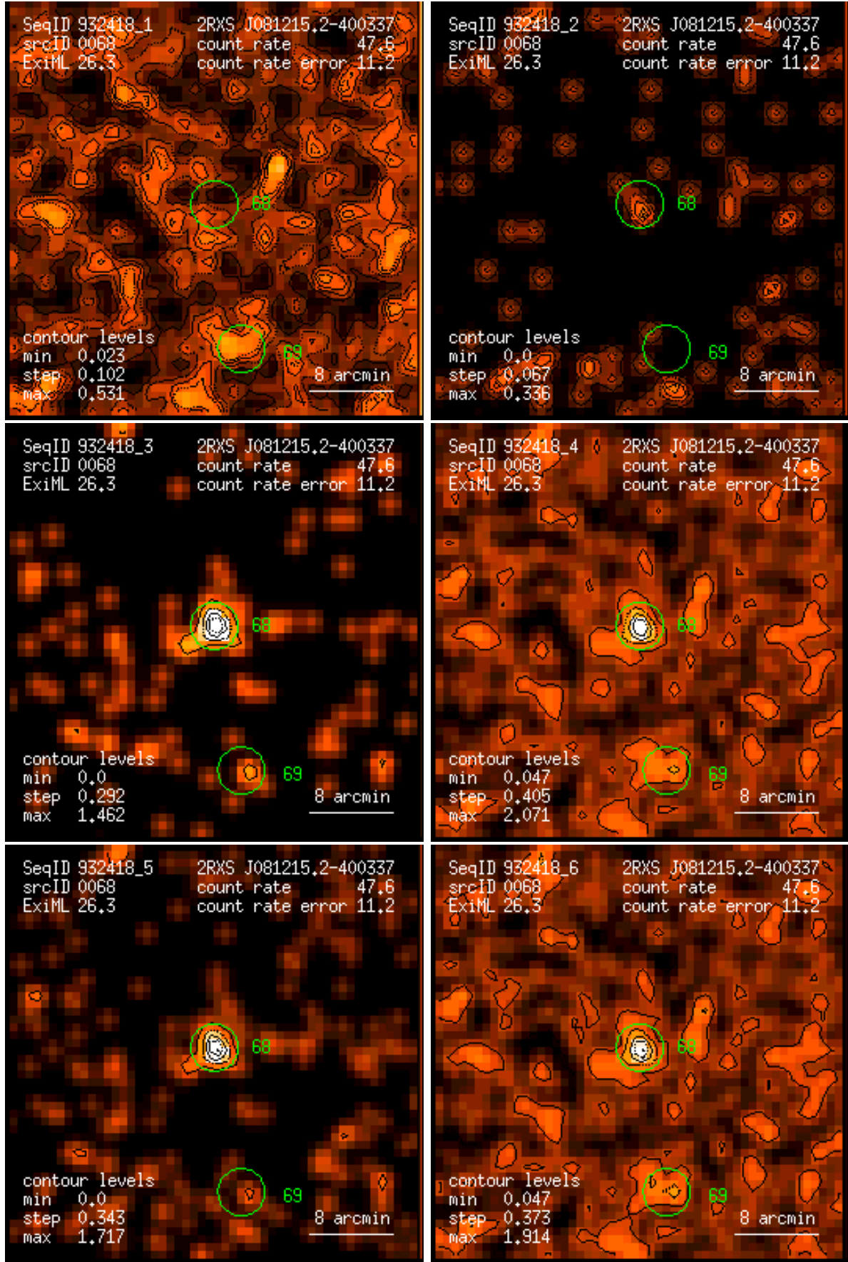
Figure 68: RASS 932418: detection 0068: band rate images, Gaussian filter: (1) PSPC channels 11 – 41, (2) 52 – 90, (3) 91 – 201, (4) 11 – 235, (5) 52 – 201, (6) 11 – 201. Broad band rates in counts/ks. Band rate contour levels in counts/ks/arcmin 2 .
