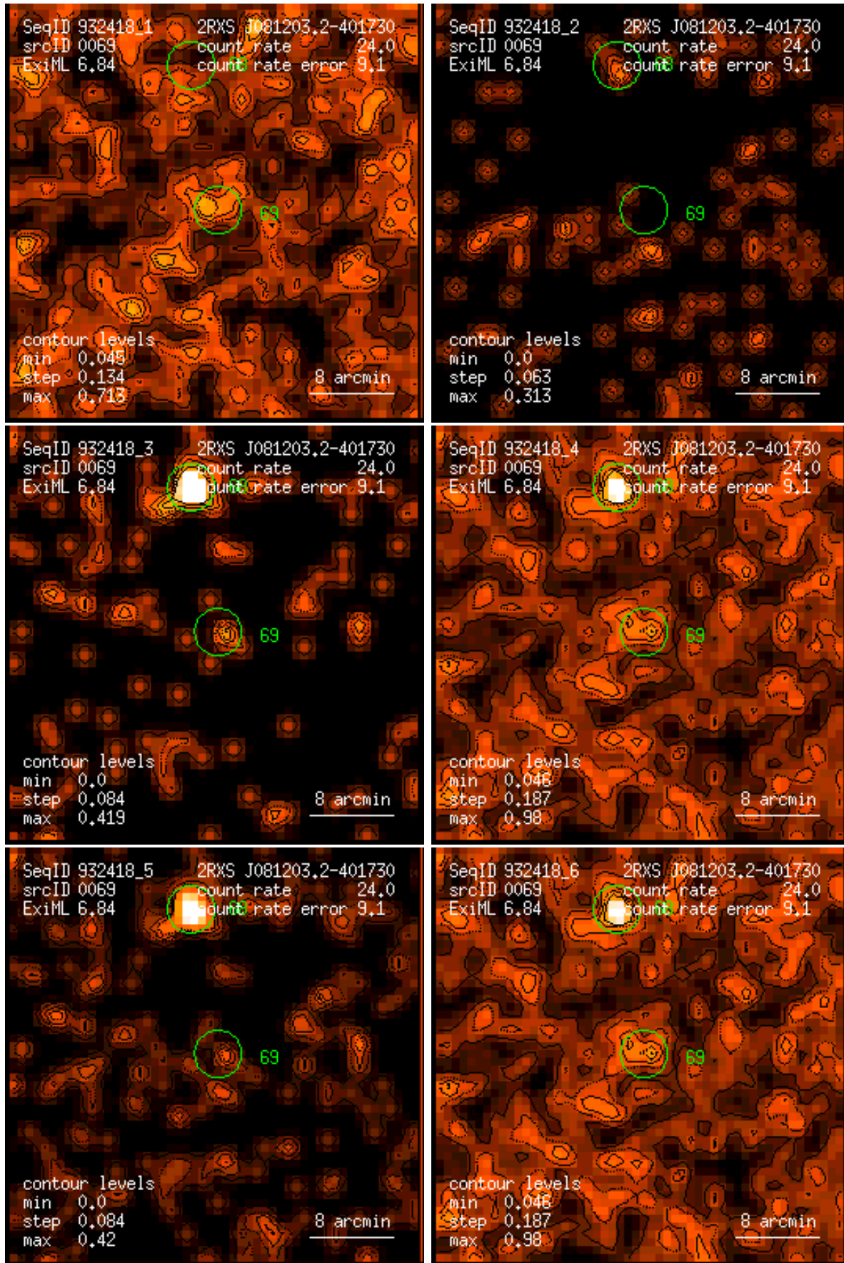
Figure 69: RASS 932418: detection 0069: band rate images, Gaussian filter: (1) PSPC channels 11 – 41, (2) 52 – 90, (3) 91 – 201, (4) 11 – 235, (5) 52 – 201, (6) 11 – 201. Broad band rates in counts/ks. Band rate contour levels in counts/ks/arcmin 2 .
