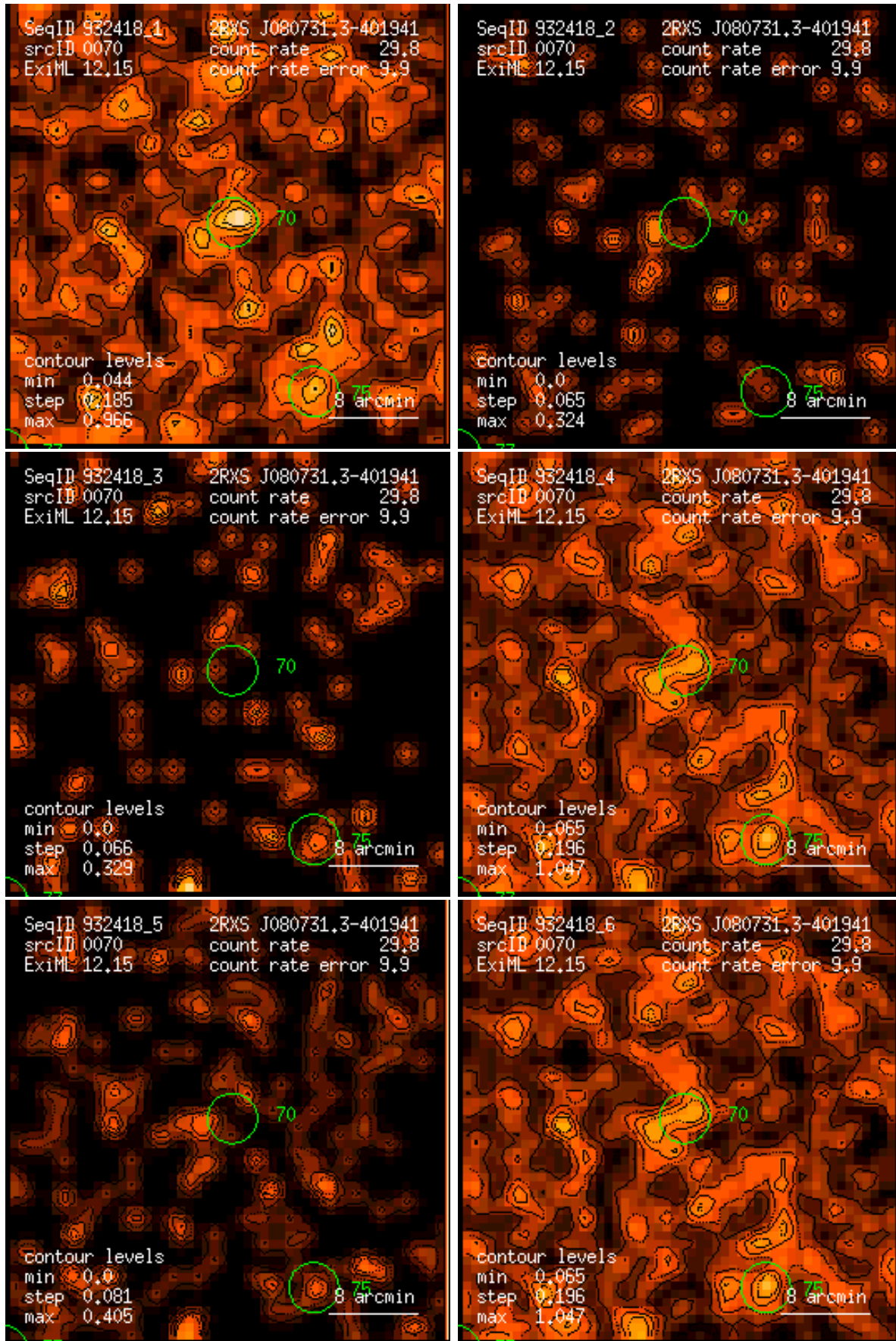
Figure 70: RASS 932418: detection 0070: band rate images, Gaussian filter: (1) PSPC channels 11 – 41, (2) 52 – 90, (3) 91 – 201, (4) 11 – 235, (5) 52 – 201, (6) 11 – 201. Broad band rates in counts/ks. Band rate contour levels in counts/ks/arcmin 2 .
