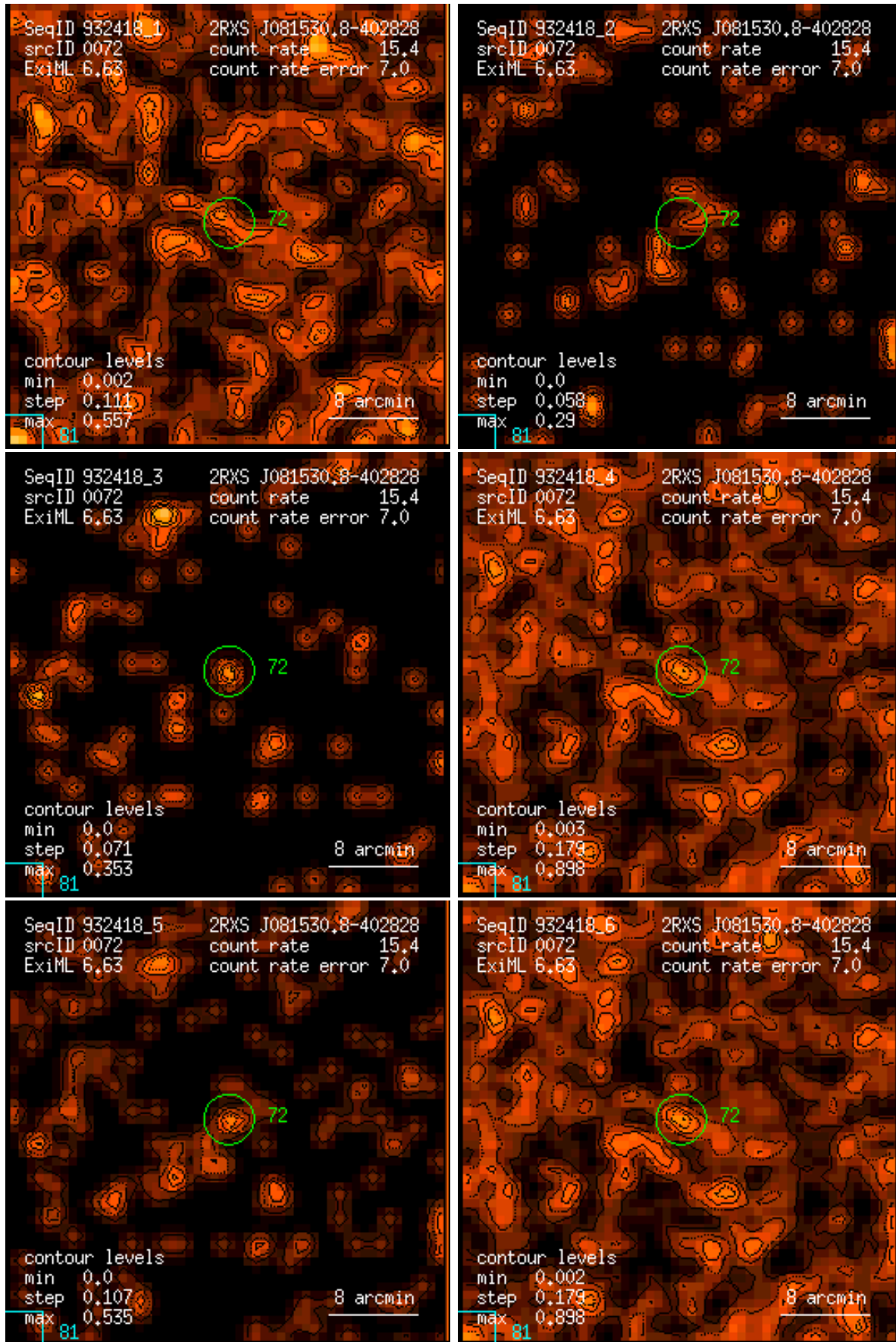
Figure 72: RASS 932418: detection 0072: band rate images, Gaussian filter: (1) PSPC channels 11 – 41, (2) 52 – 90, (3) 91 – 201, (4) 11 – 235, (5) 52 – 201, (6) 11 – 201. Broad band rates in counts/ks. Band rate contour levels in counts/ks/arcmin 2 .
