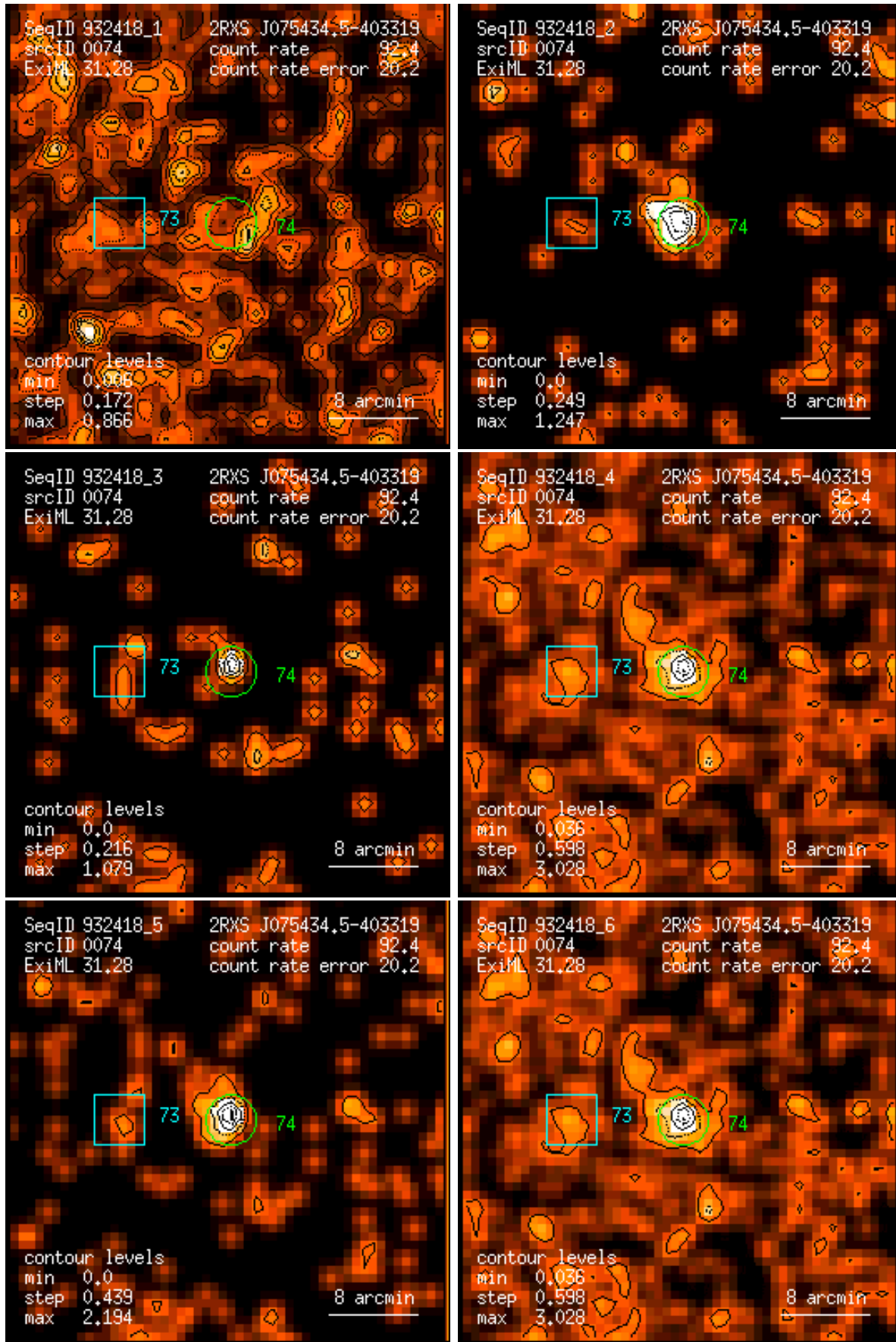
Figure 74: RASS 932418: detection 0074: band rate images, Gaussian filter: (1) PSPC channels 11 – 41, (2) 52 – 90, (3) 91 – 201, (4) 11 – 235, (5) 52 – 201, (6) 11 – 201. Broad band rates in counts/ks. Band rate contour levels in counts/ks/arcmin 2 .
