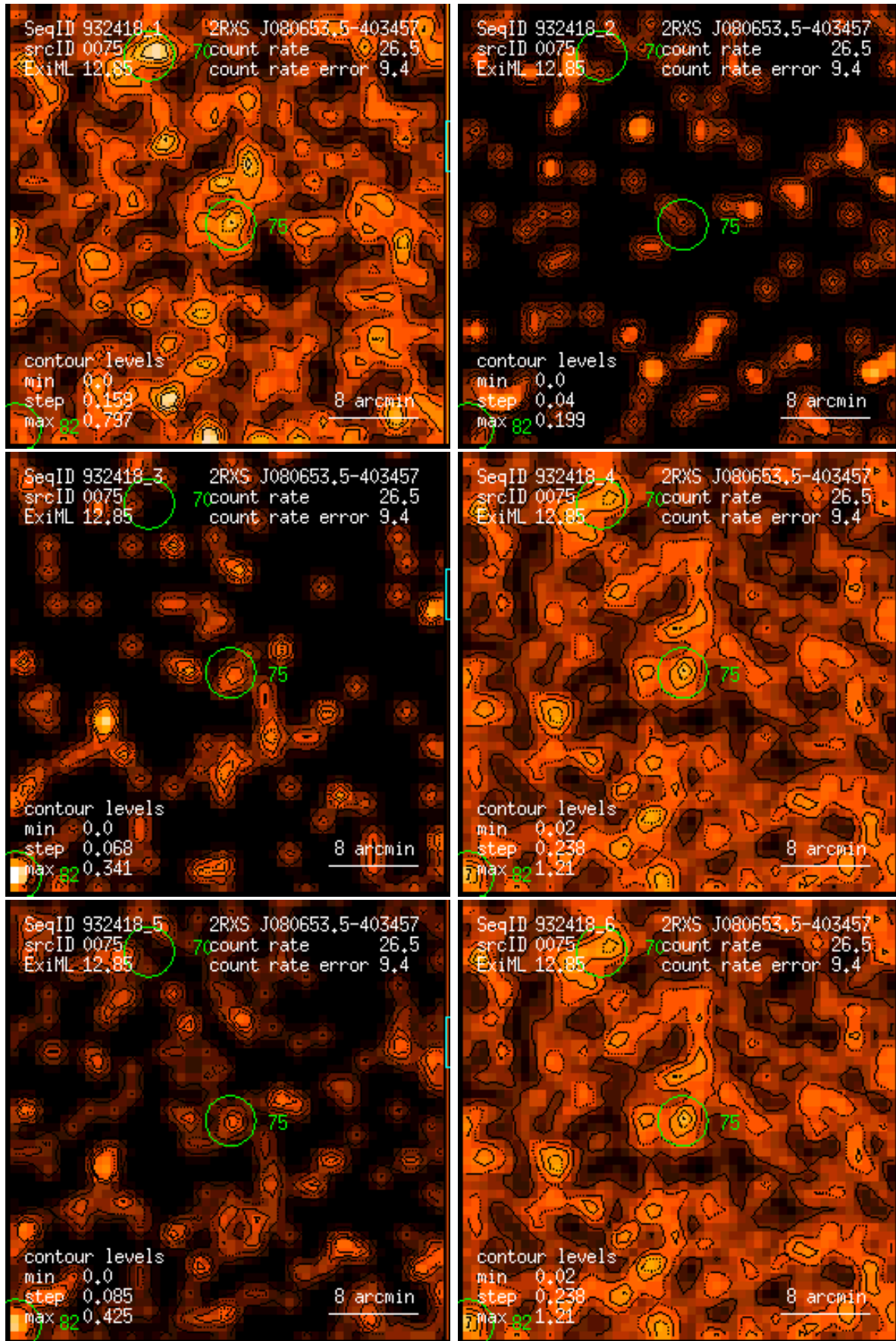
Figure 75: RASS 932418: detection 0075: band rate images, Gaussian filter: (1) PSPC channels 11 – 41, (2) 52 – 90, (3) 91 – 201, (4) 11 – 235, (5) 52 – 201, (6) 11 – 201. Broad band rates in counts/ks. Band rate contour levels in counts/ks/arcmin 2 .
