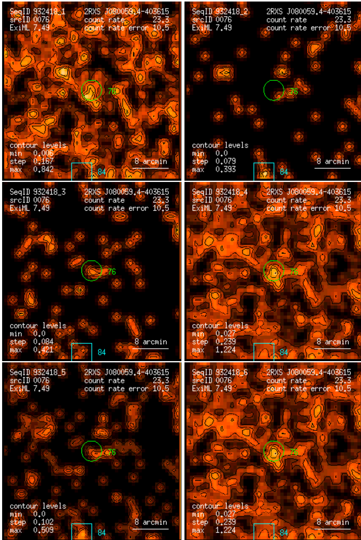
Figure 76: RASS 932418: detection 0076: band rate images, Gaussian filter: (1) PSPC channels 11 – 41, (2) 52 – 90, (3) 91 – 201, (4) 11 – 235, (5) 52 – 201, (6) 11 – 201. Broad band rates in counts/ks. Band rate contour levels in counts/ks/arcmin 2 .
