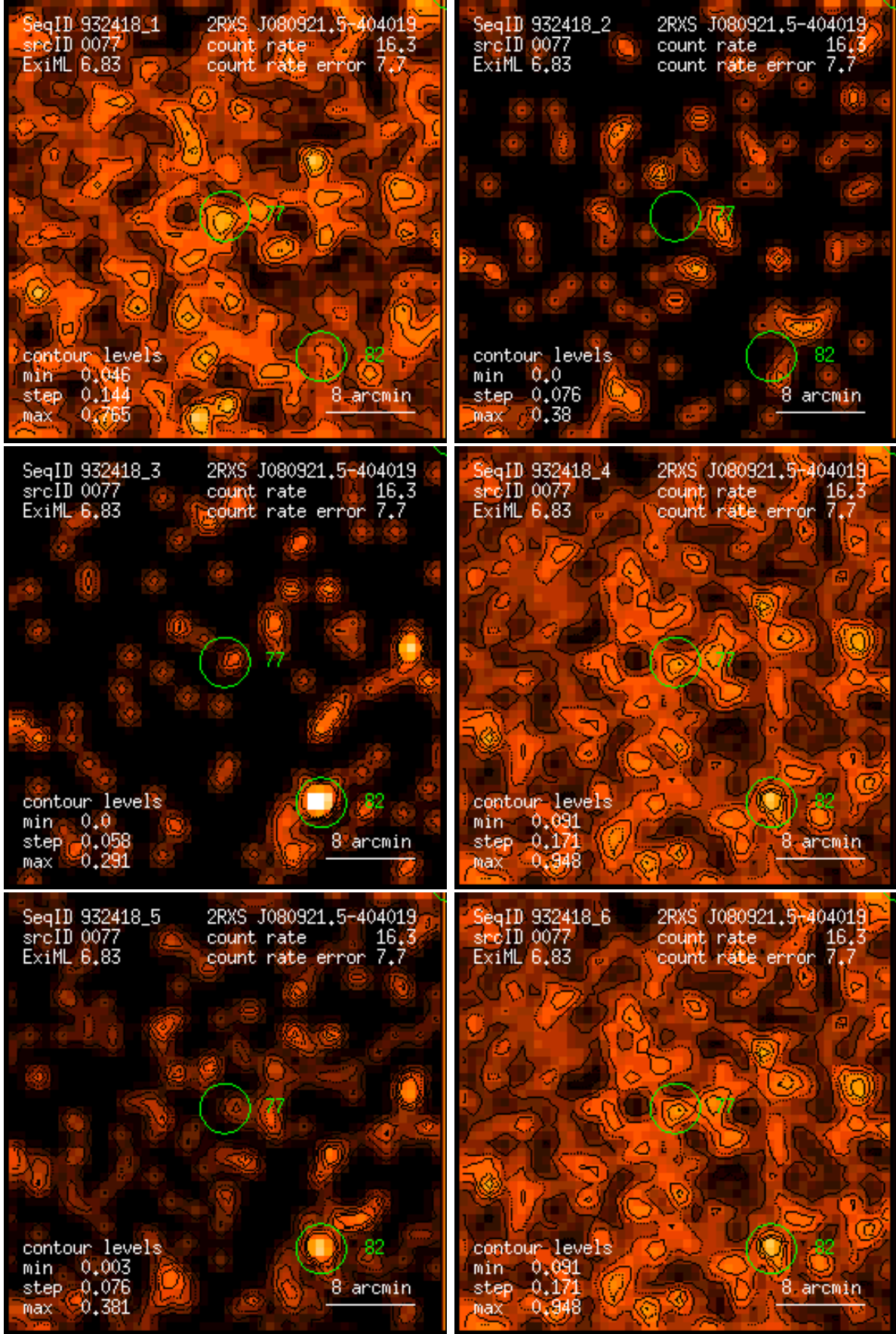
Figure 77: RASS 932418: detection 0077: band rate images, Gaussian filter: (1) PSPC channels 11 – 41, (2) 52 – 90, (3) 91 – 201, (4) 11 – 235, (5) 52 – 201, (6) 11 – 201. Broad band rates in counts/ks. Band rate contour levels in counts/ks/arcmin 2 .
