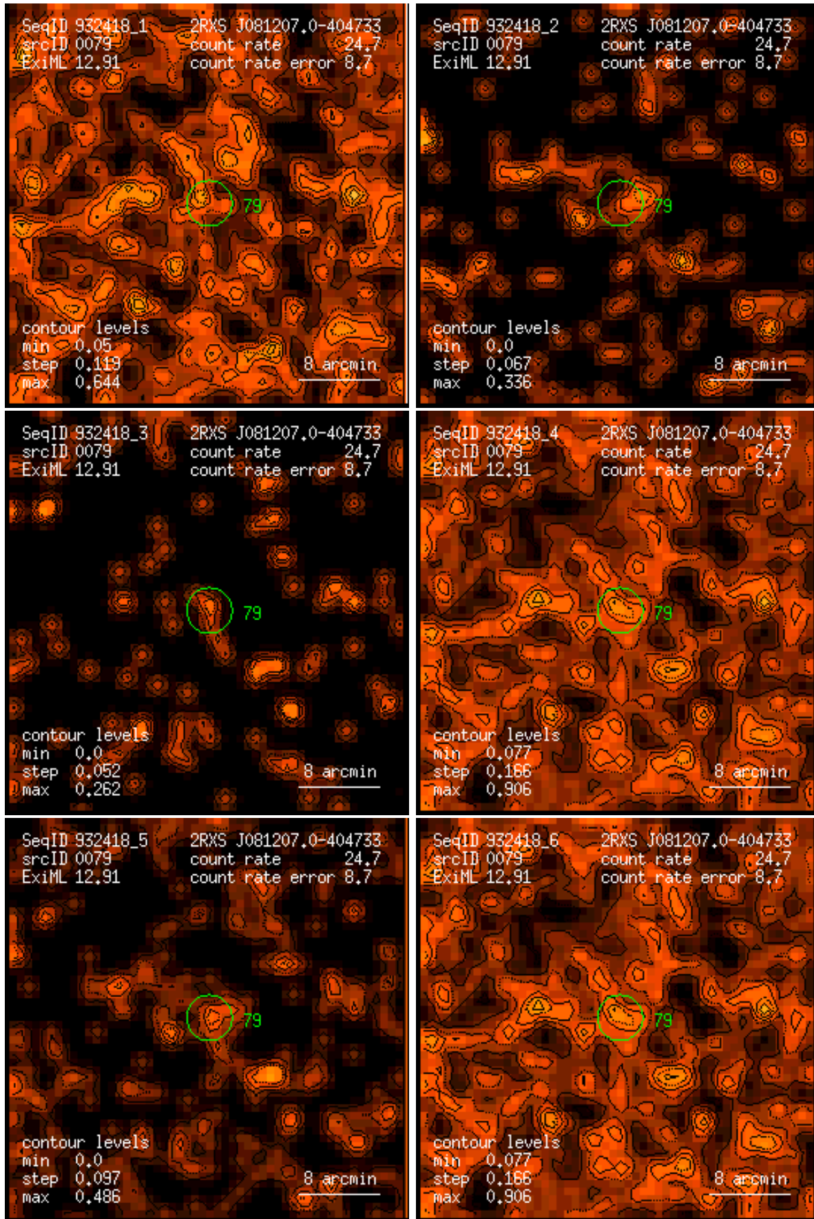
Figure 79: RASS 932418: detection 0079: band rate images, Gaussian filter: (1) PSPC channels 11 – 41, (2) 52 – 90, (3) 91 – 201, (4) 11 – 235, (5) 52 – 201, (6) 11 – 201. Broad band rates in counts/ks. Band rate contour levels in counts/ks/arcmin 2 .
