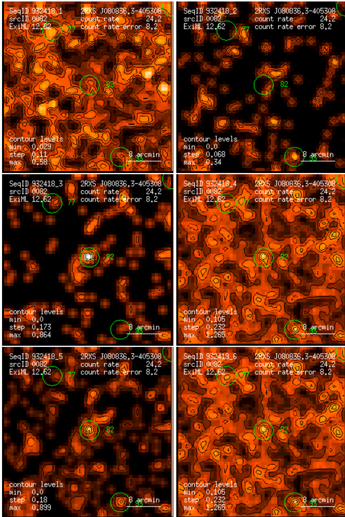
Figure 82: RASS 932418: detection 0082: band rate images, Gaussian filter: (1) PSPC channels 11 – 41, (2) 52 – 90, (3) 91 – 201, (4) 11 – 235, (5) 52 – 201, (6) 11 – 201. Broad band rates in counts/ks. Band rate contour levels in counts/ks/arcmin 2 .
