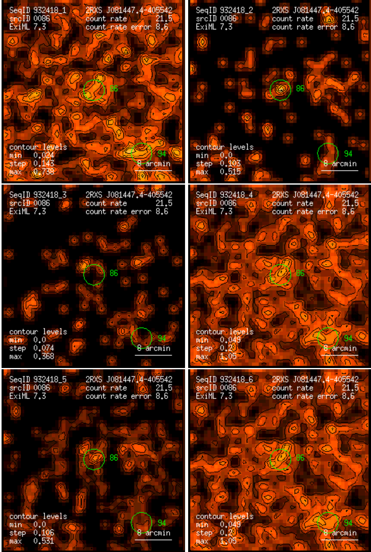
Figure 86: RASS 932418: detection 0086: band rate images, Gaussian filter: (1) PSPC channels 11 – 41, (2) 52 – 90, (3) 91 – 201, (4) 11 – 235, (5) 52 – 201, (6) 11 – 201. Broad band rates in counts/ks. Band rate contour levels in counts/ks/arcmin 2 .
