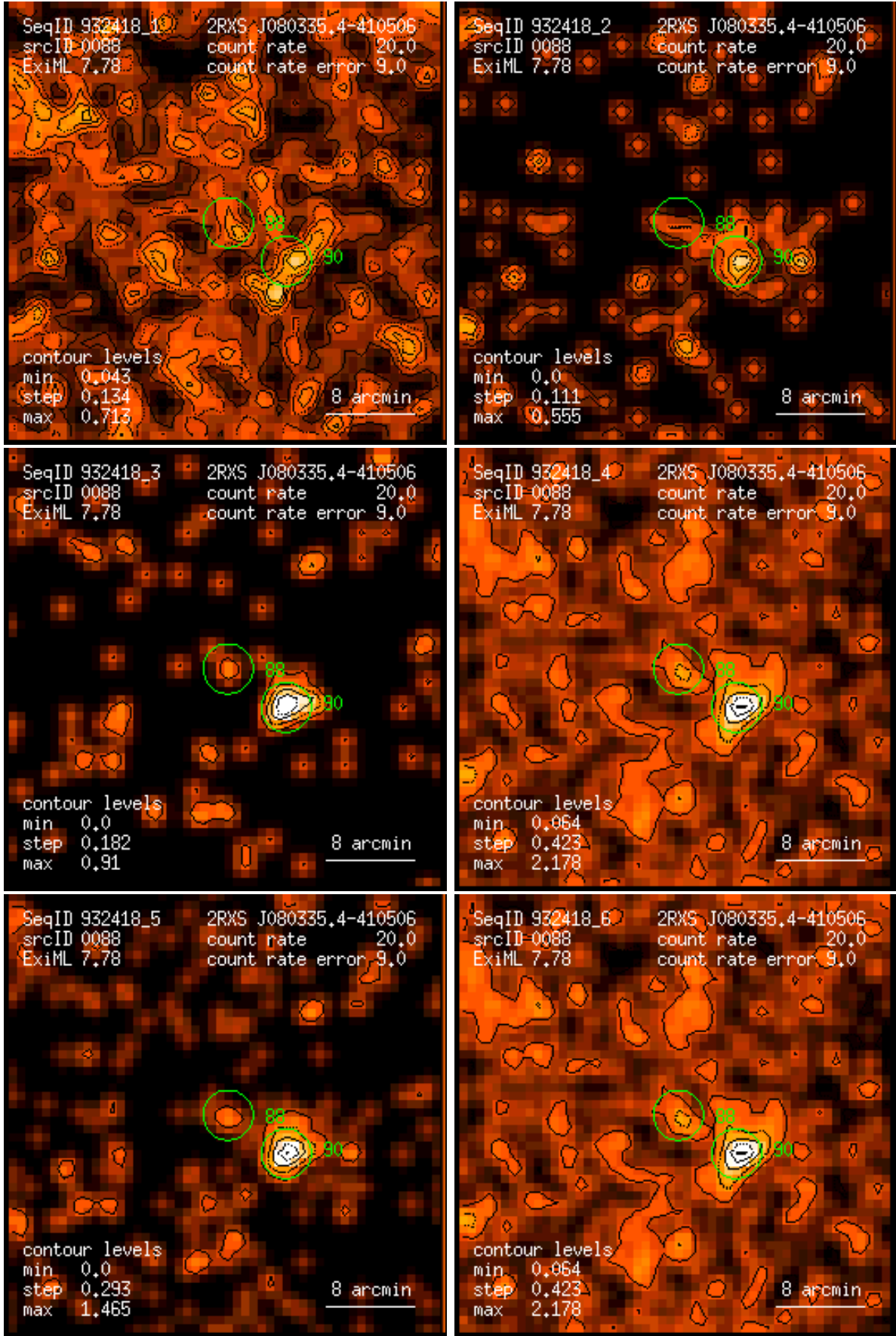
Figure 88: RASS 932418: detection 0088: band rate images, Gaussian filter: (1) PSPC channels 11 – 41, (2) 52 – 90, (3) 91 – 201, (4) 11 – 235, (5) 52 – 201, (6) 11 – 201. Broad band rates in counts/ks. Band rate contour levels in counts/ks/arcmin 2 .
