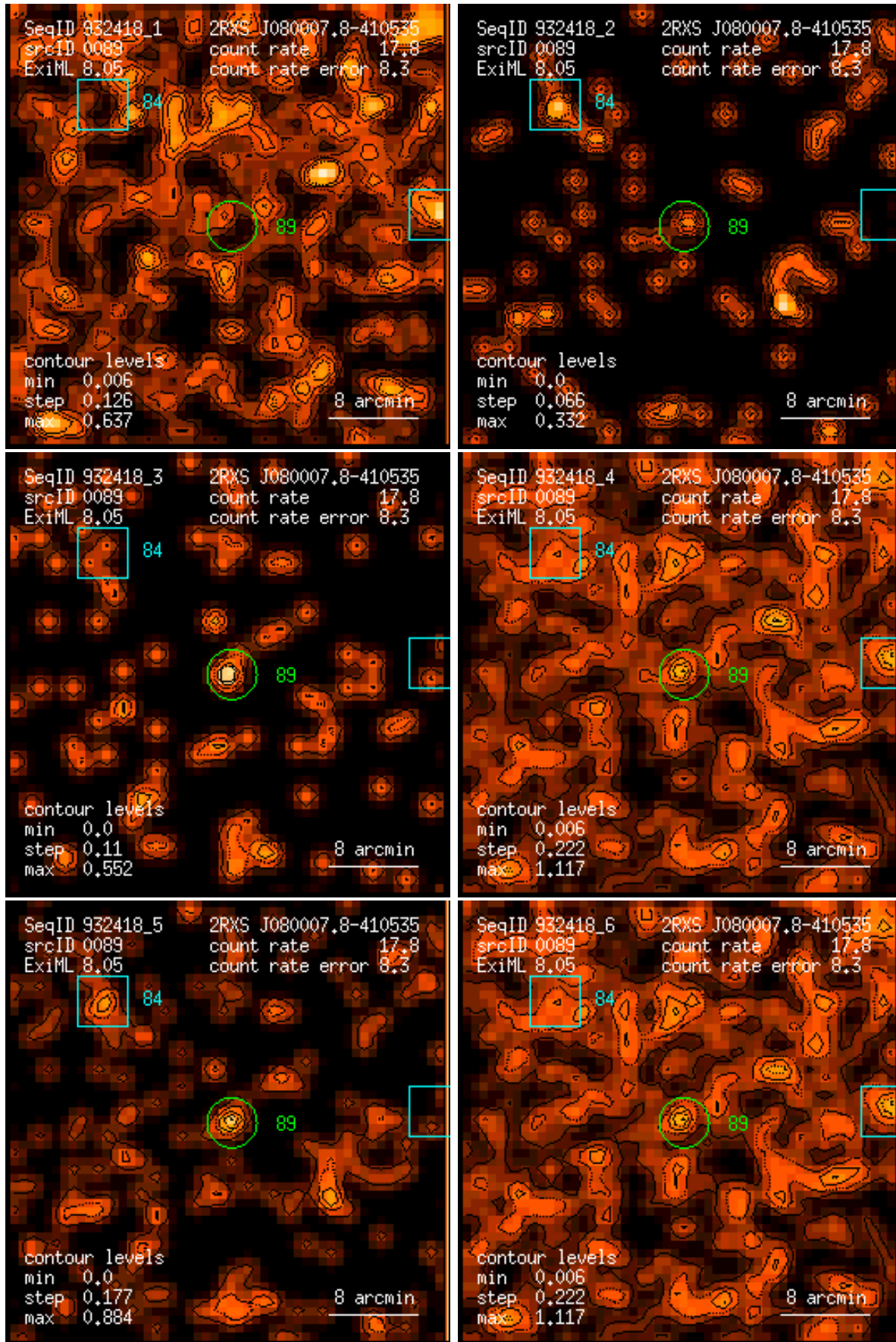
Figure 89: RASS 932418: detection 0089: band rate images, Gaussian filter: (1) PSPC channels 11 – 41, (2) 52 – 90, (3) 91 – 201, (4) 11 – 235, (5) 52 – 201, (6) 11 – 201. Broad band rates in counts/ks. Band rate contour levels in counts/ks/arcmin 2 .
