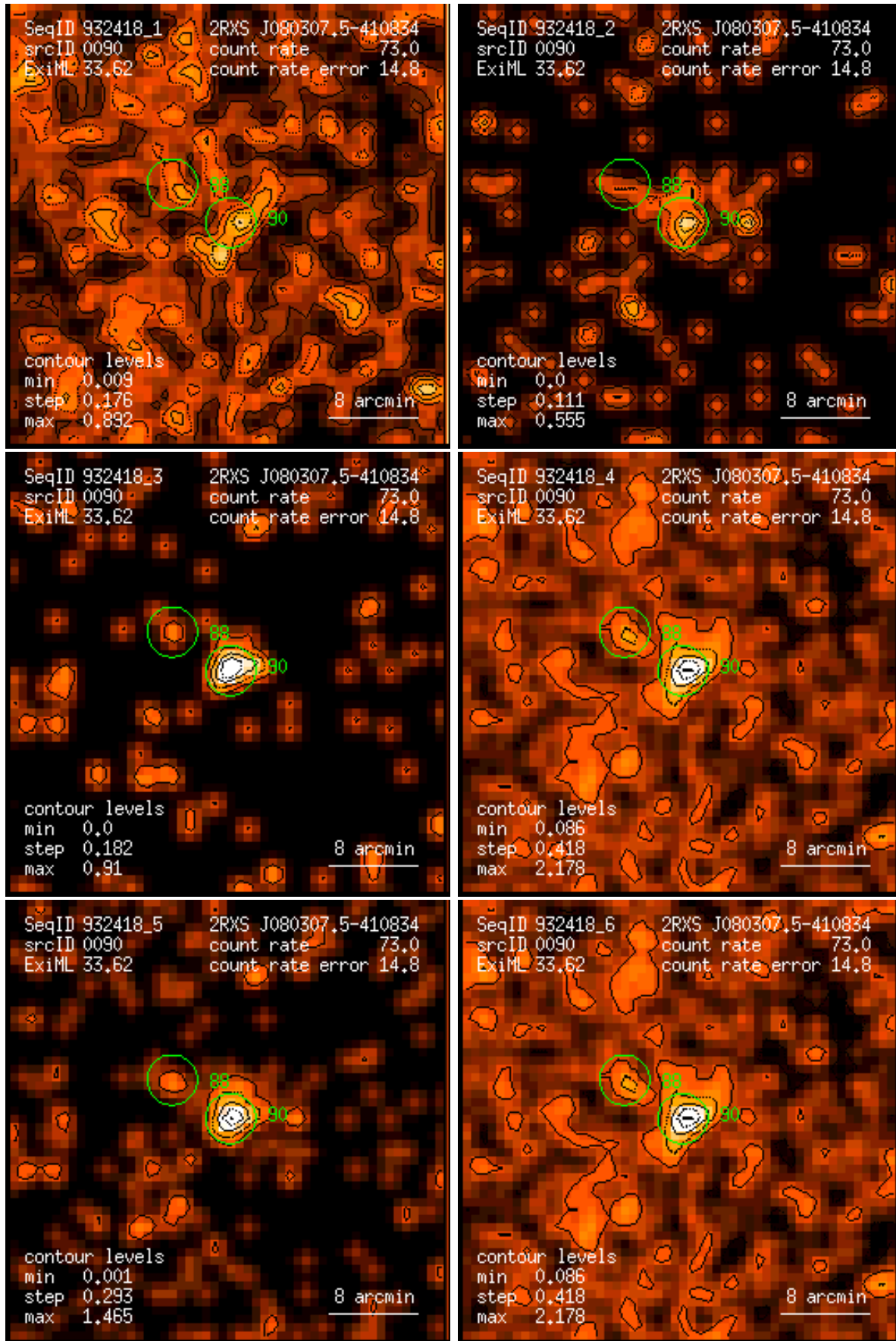
Figure 90: RASS 932418: detection 0090: band rate images, Gaussian filter: (1) PSPC channels 11 – 41, (2) 52 – 90, (3) 91 – 201, (4) 11 – 235, (5) 52 – 201, (6) 11 – 201. Broad band rates in counts/ks. Band rate contour levels in counts/ks/arcmin 2 .
