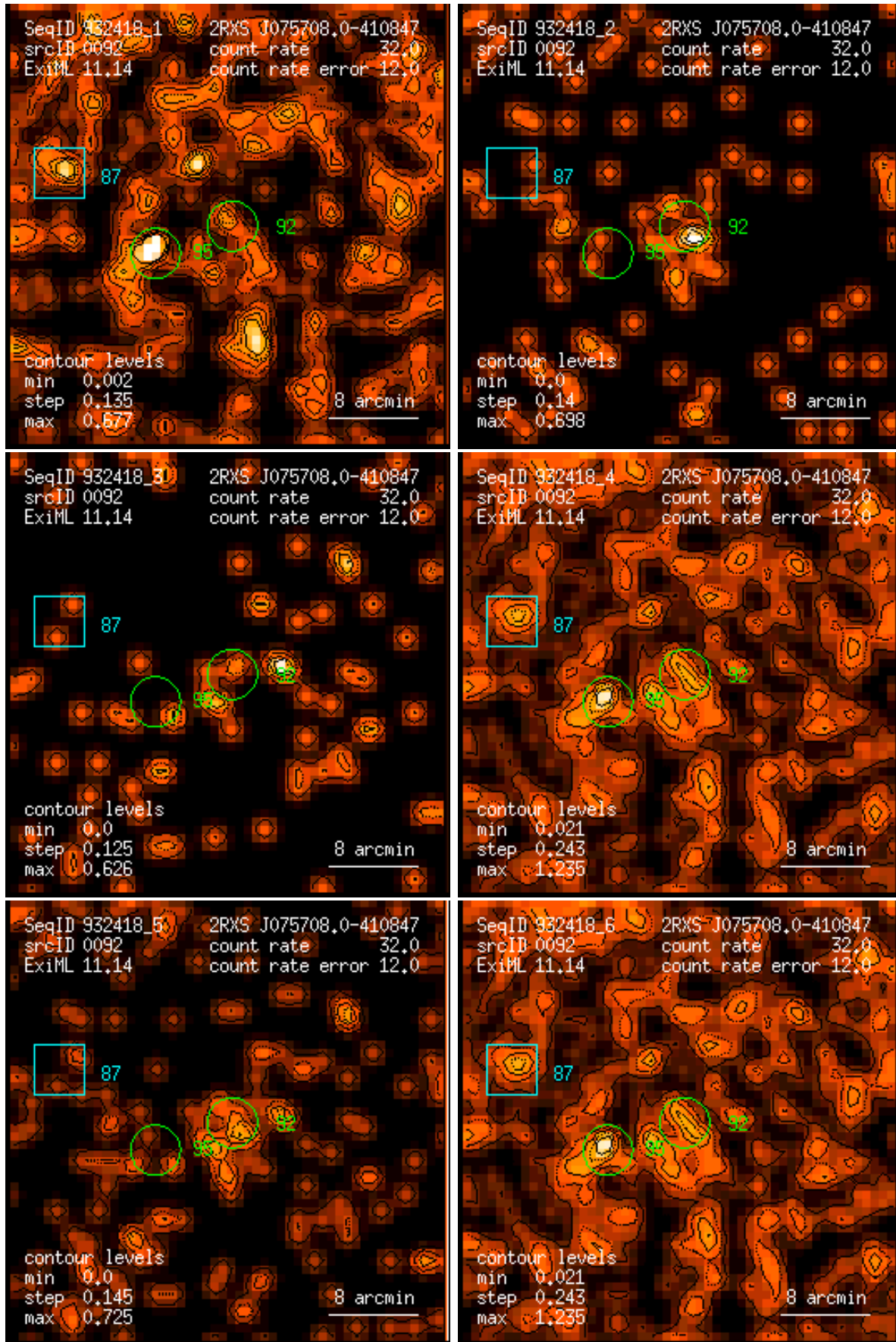
Figure 92: RASS 932418: detection 0092: band rate images, Gaussian filter: (1) PSPC channels 11 – 41, (2) 52 – 90, (3) 91 – 201, (4) 11 – 235, (5) 52 – 201, (6) 11 – 201. Broad band rates in counts/ks. Band rate contour levels in counts/ks/arcmin 2 .
