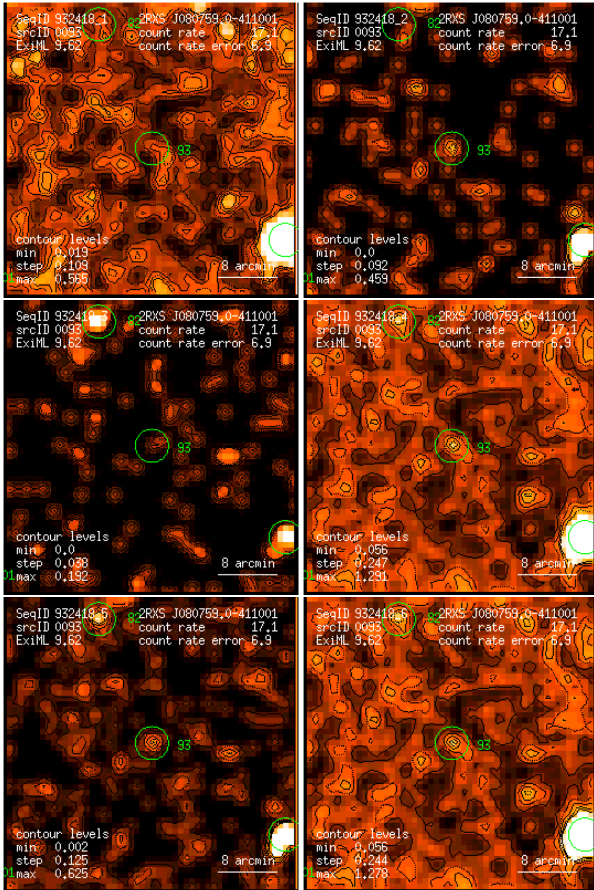
Figure 93: RASS 932418: detection 0093: band rate images, Gaussian filter: (1) PSPC channels 11 – 41, (2) 52 – 90, (3) 91 – 201, (4) 11 – 235, (5) 52 – 201, (6) 11 – 201. Broad band rates in counts/ks. Band rate contour levels in counts/ks/arcmin 2 .
