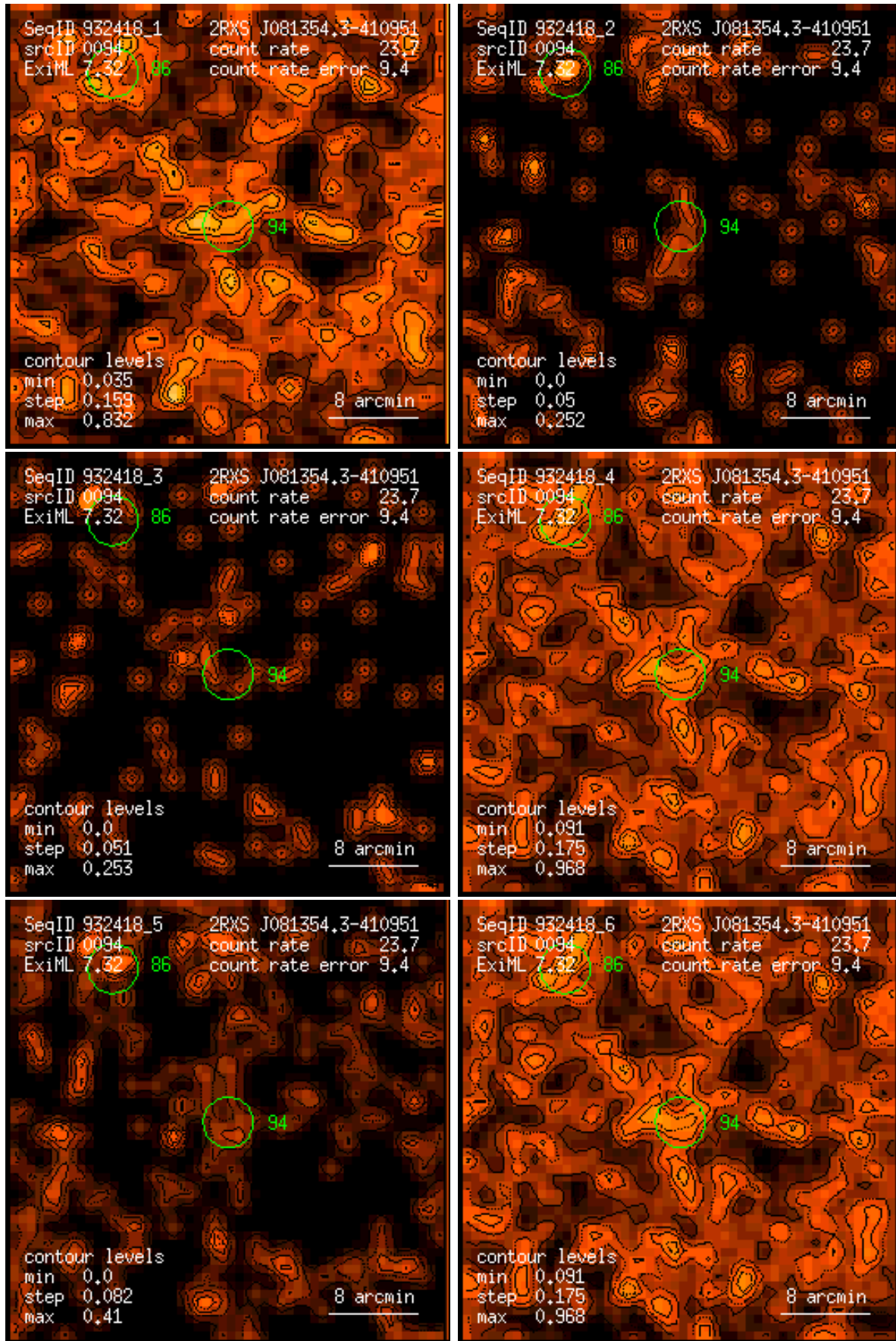
Figure 94: RASS 932418: detection 0094: band rate images, Gaussian filter: (1) PSPC channels 11 – 41, (2) 52 – 90, (3) 91 – 201, (4) 11 – 235, (5) 52 – 201, (6) 11 – 201. Broad band rates in counts/ks. Band rate contour levels in counts/ks/arcmin 2 .
