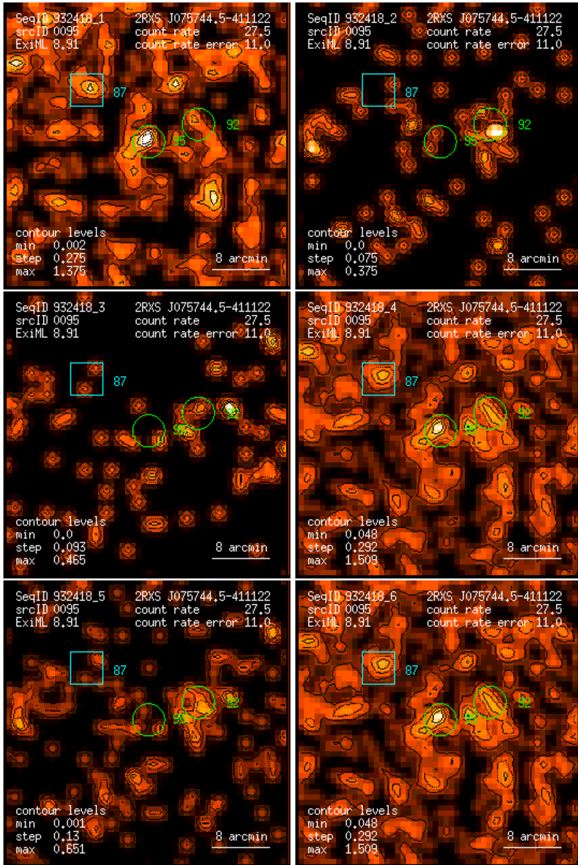
Figure 95: RASS 932418: detection 0095: band rate images, Gaussian filter: (1) PSPC channels 11 – 41, (2) 52 – 90, (3) 91 – 201, (4) 11 – 235, (5) 52 – 201, (6) 11 – 201. Broad band rates in counts/ks. Band rate contour levels in counts/ks/arcmin 2 .
