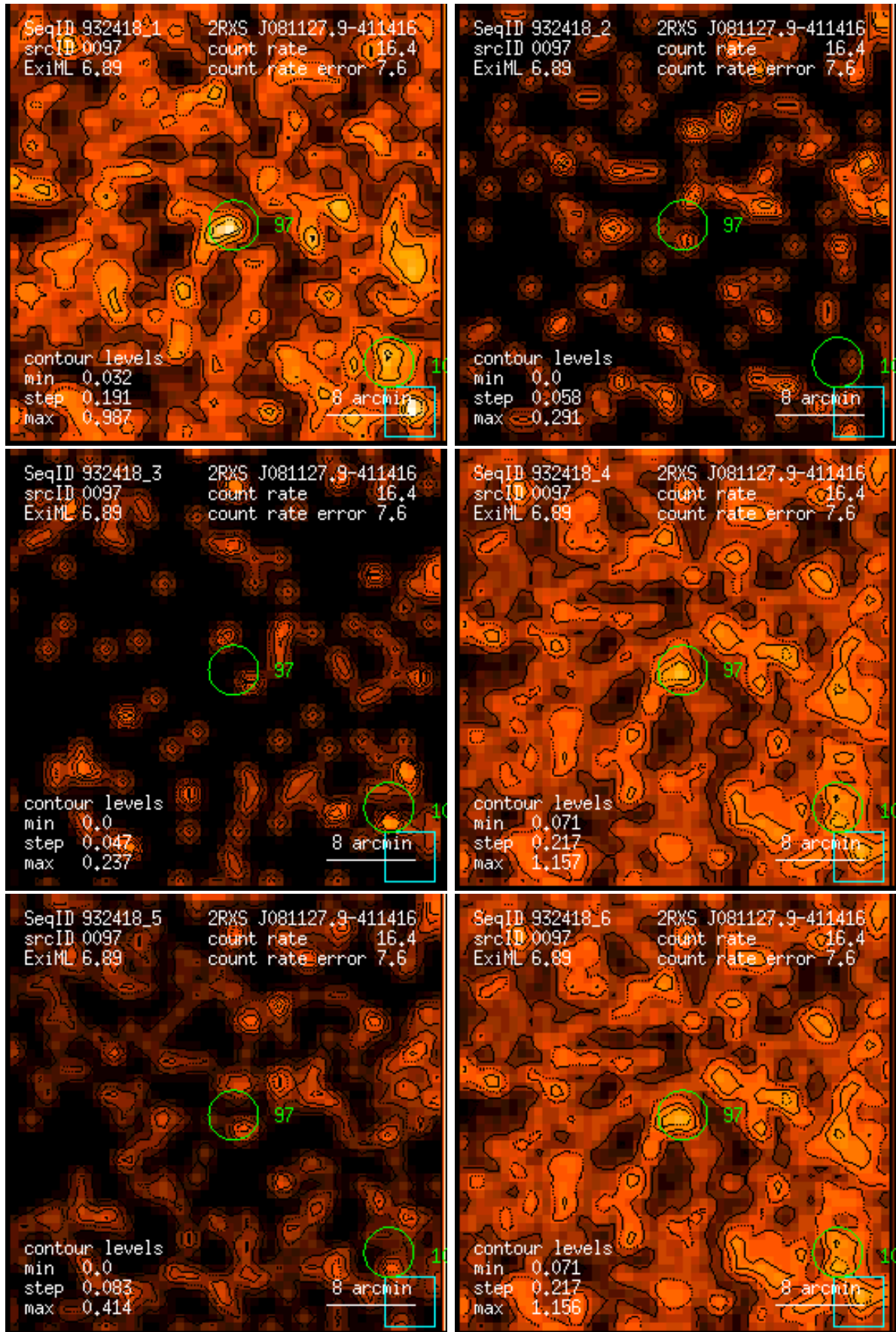
Figure 97: RASS 932418: detection 0097: band rate images, Gaussian filter: (1) PSPC channels 11 – 41, (2) 52 – 90, (3) 91 – 201, (4) 11 – 235, (5) 52 – 201, (6) 11 – 201. Broad band rates in counts/ks. Band rate contour levels in counts/ks/arcmin 2 .
