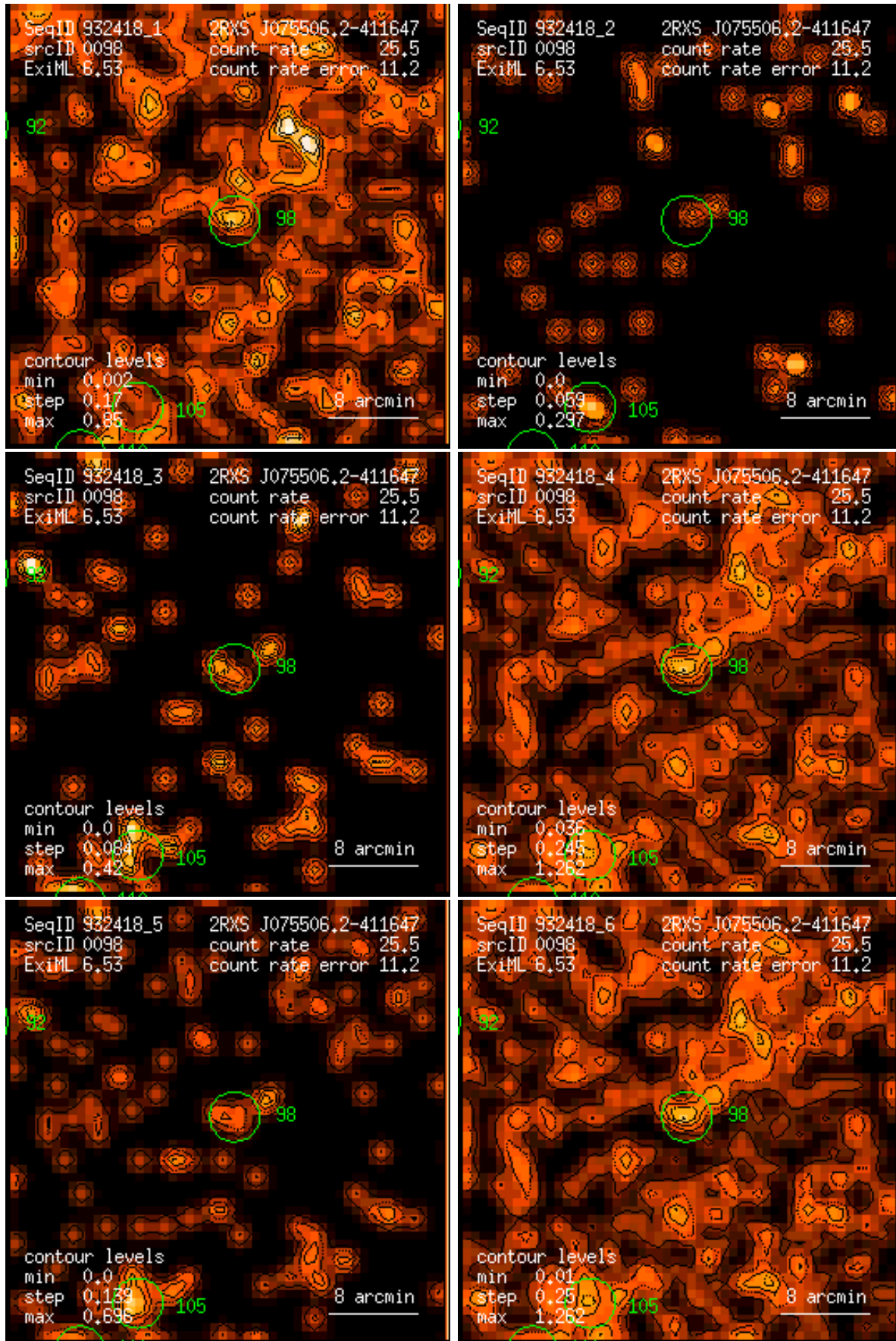
Figure 98: RASS 932418: detection 0098: band rate images, Gaussian filter: (1) PSPC channels 11 – 41, (2) 52 – 90, (3) 91 – 201, (4) 11 – 235, (5) 52 – 201, (6) 11 – 201. Broad band rates in counts/ks. Band rate contour levels in counts/ks/arcmin 2 .
