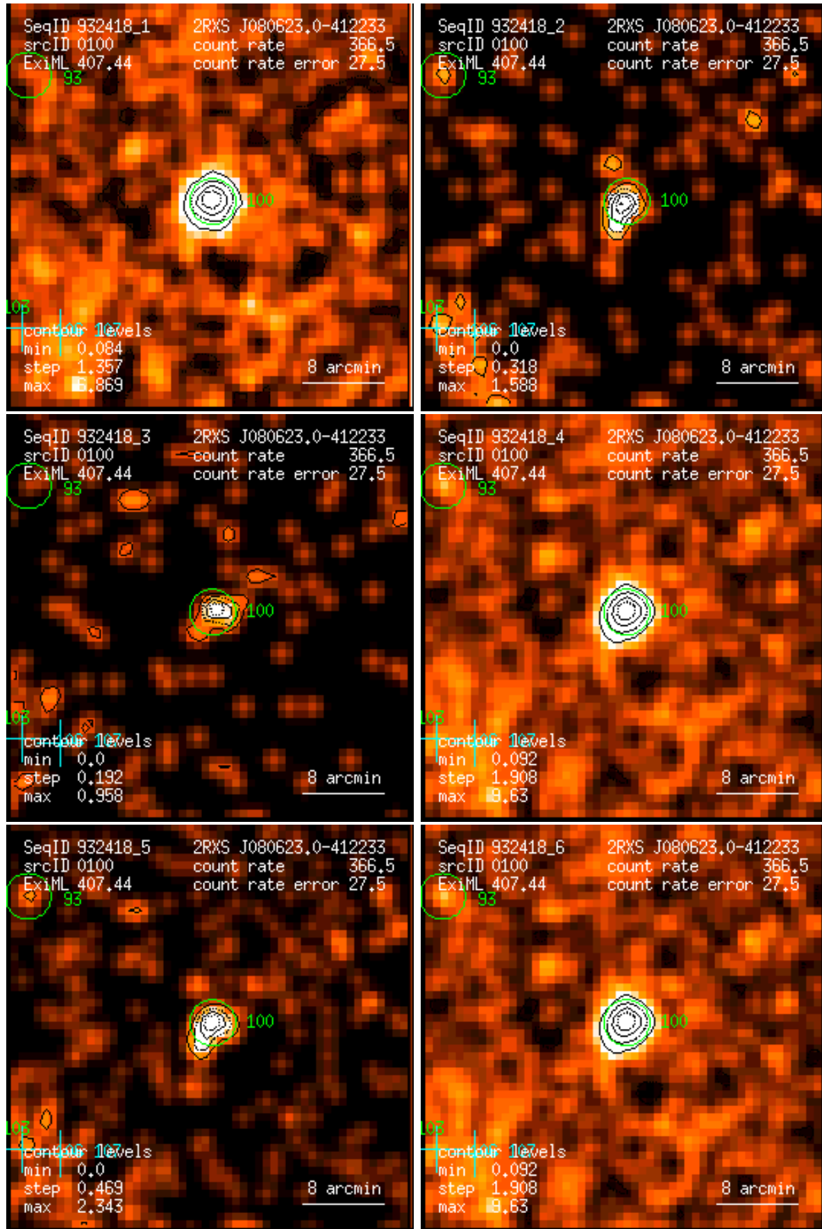
Figure 100: RASS 932418: detection 0100: band rate images, Gaussian filter: (1) PSPC channels 11 – 41, (2) 52 – 90, (3) 91 – 201, (4) 11 – 235, (5) 52 – 201, (6) 11 – 201. Broad band rates in counts/ks. Band rate contour levels in counts/ks/arcmin 2 .
