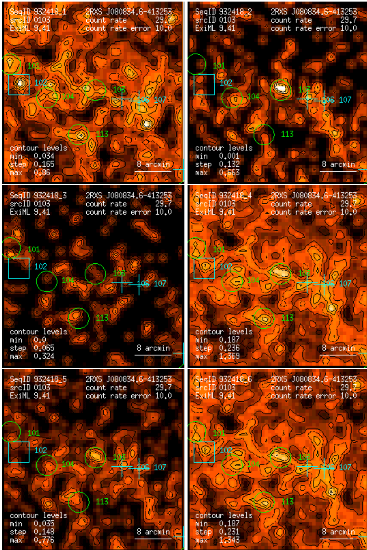
Figure 103: RASS 932418: detection 0103: band rate images, Gaussian filter: (1) PSPC channels 11 – 41, (2) 52 – 90, (3) 91 – 201, (4) 11 – 235, (5) 52 – 201, (6) 11 – 201. Broad band rates in counts/ks. Band rate contour levels in counts/ks/arcmin 2 .
