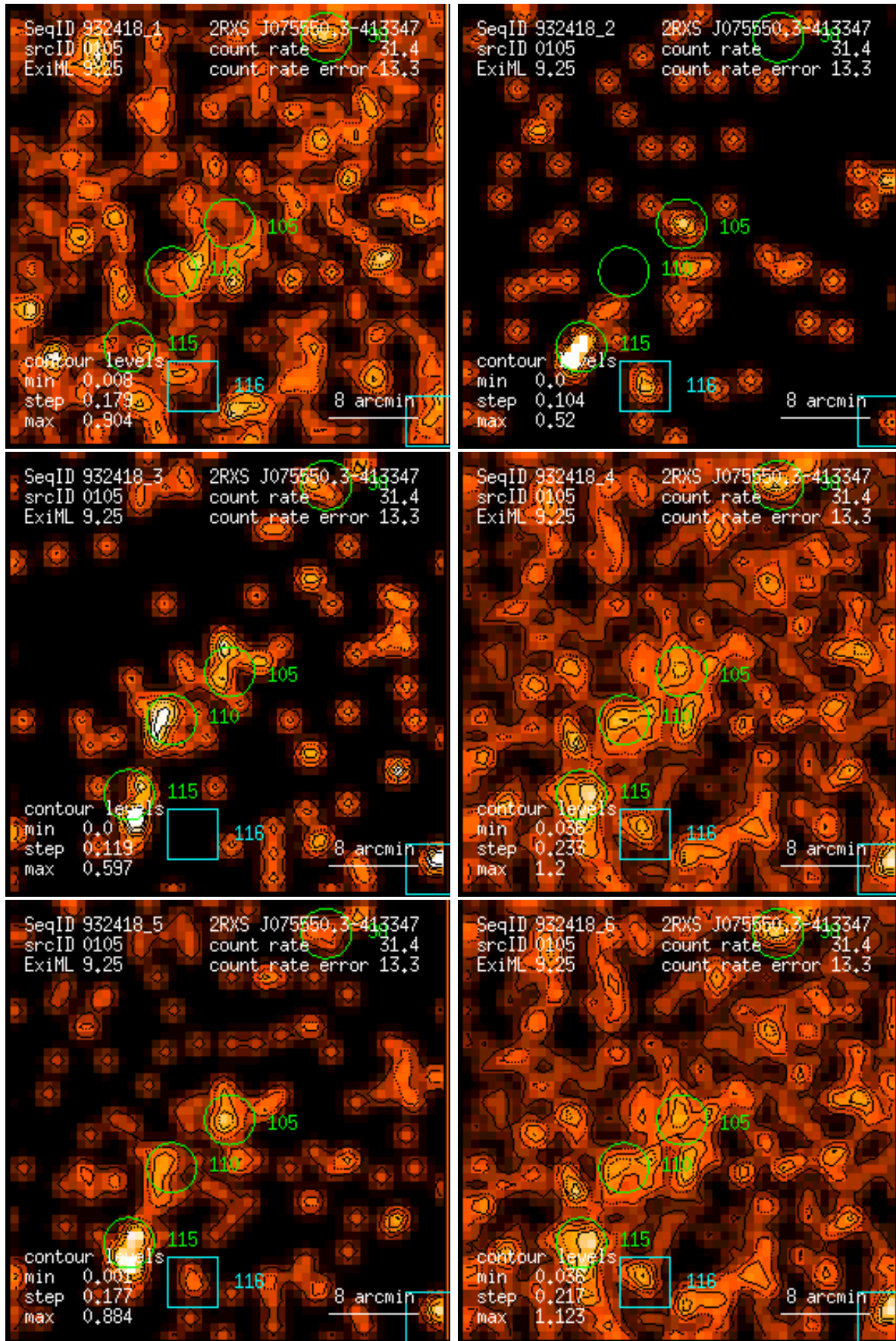
Figure 105: RASS 932418: detection 0105: band rate images, Gaussian filter: (1) PSPC channels 11 – 41, (2) 52 – 90, (3) 91 – 201, (4) 11 – 235, (5) 52 – 201, (6) 11 – 201. Broad band rates in counts/ks. Band rate contour levels in counts/ks/arcmin 2 .
