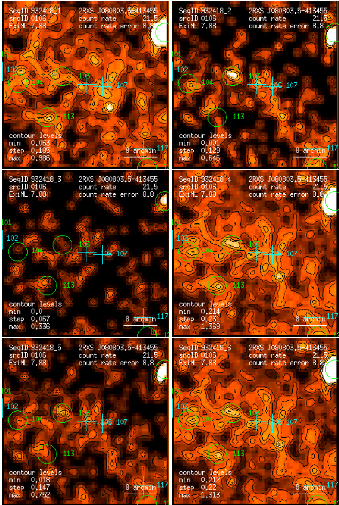
Figure 106: RASS 932418: detection 0106: band rate images, Gaussian filter: (1) PSPC channels 11 – 41, (2) 52 – 90, (3) 91 – 201, (4) 11 – 235, (5) 52 – 201, (6) 11 – 201. Broad band rates in counts/ks. Band rate contour levels in counts/ks/arcmin 2 .
