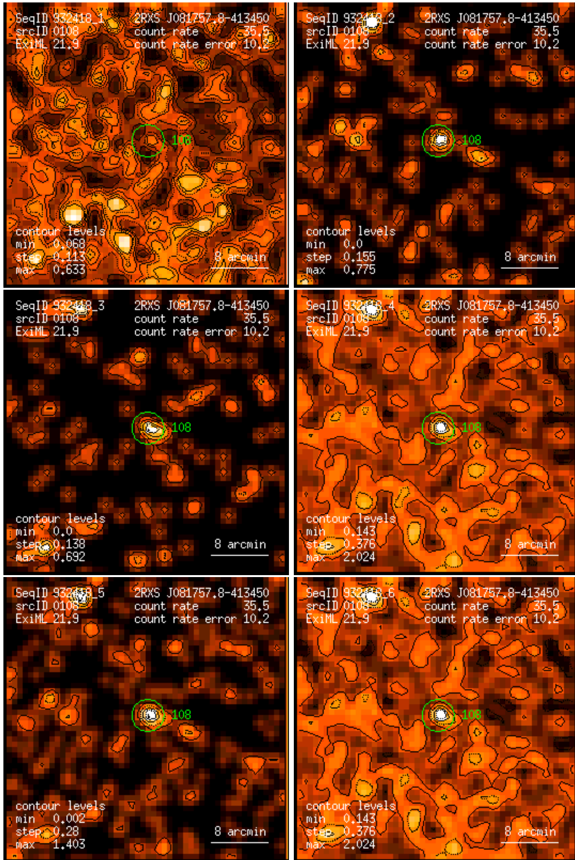
Figure 108: RASS 932418: detection 0108: band rate images, Gaussian filter: (1) PSPC channels 11 – 41, (2) 52 – 90, (3) 91 – 201, (4) 11 – 235, (5) 52 – 201, (6) 11 – 201. Broad band rates in counts/ks. Band rate contour levels in counts/ks/arcmin 2 .
